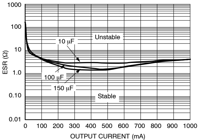
Figure 13. 1.2 Volt Output Stability with Output Capacitor ESR
