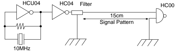
Testing Circuit
