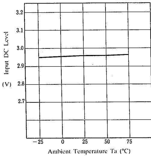
Input DC Level (Ta=25°C, V+=5V)
