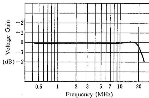
Voltage Gain
