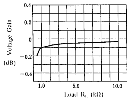
Voltage Gain
