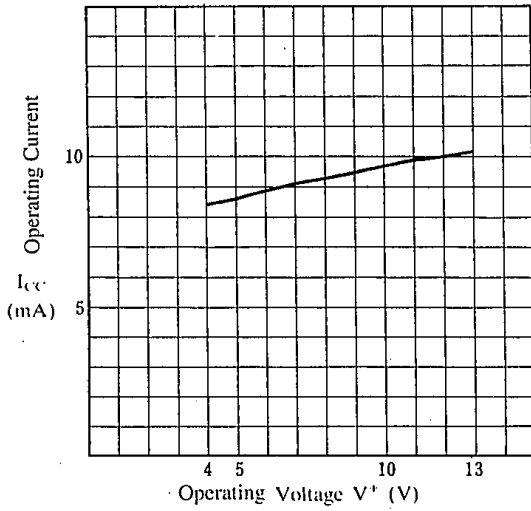
Operating Current (Ta=25°C)
