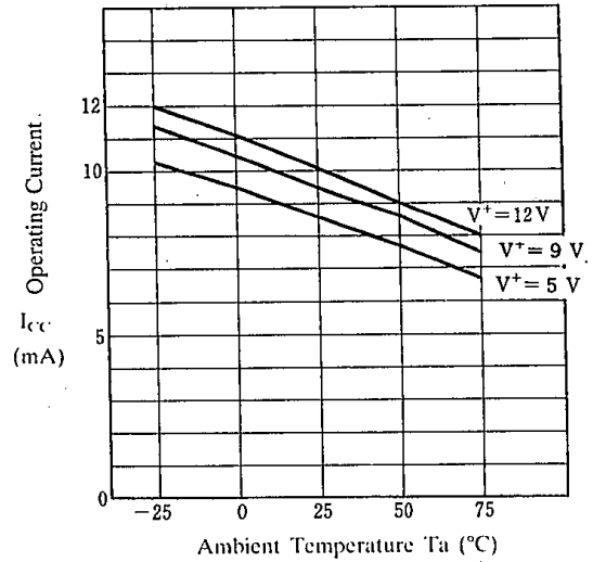
Operating Current (Ta=25°C)
