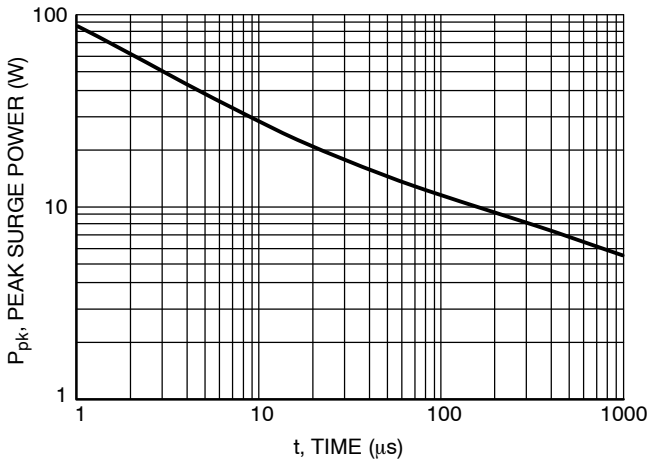
Figure 6. Pulse Width
