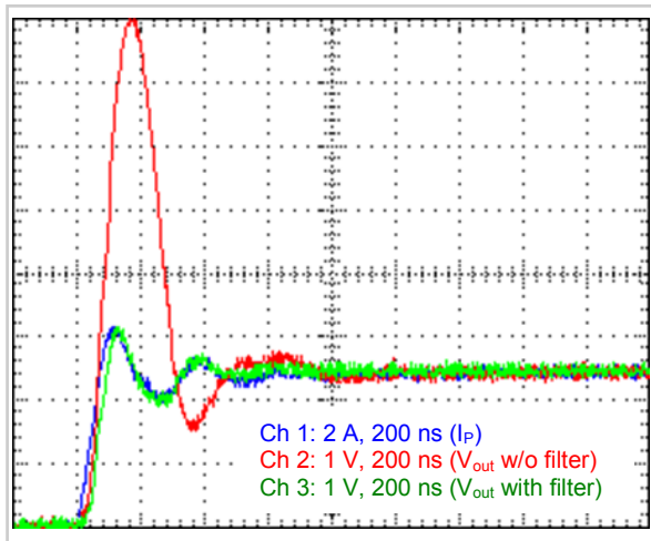
Fig. 4: Step response ( I_P = 5 \text{ A} ; di/dt \approx 70 \text{ A}/\mu\text{s} ; filter configuration acc. to Tab. 1)
