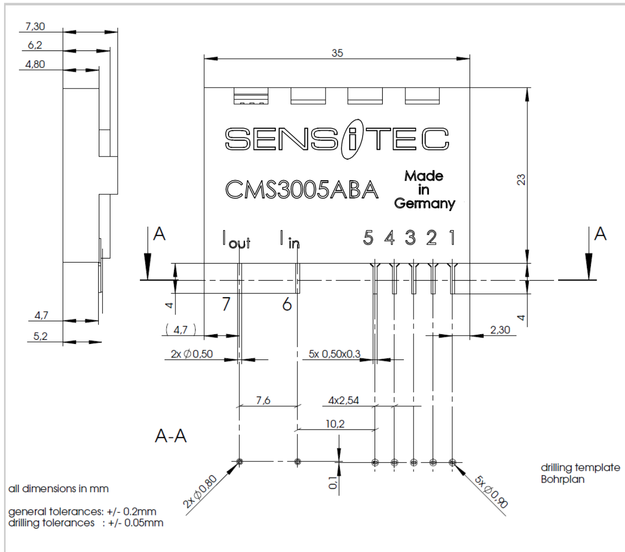
Fig.7: Package outline
