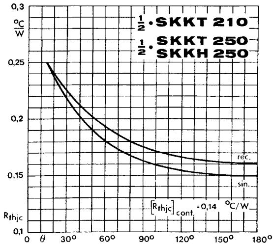
Fig. 7 Thermal resistance vs. conduction angle
