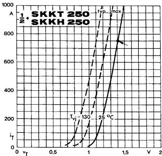
Fig. 8 b On-state characteristics
