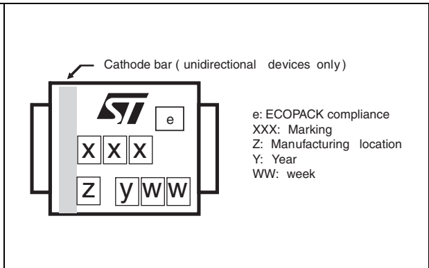
Figure 14. Marking layout (1)
