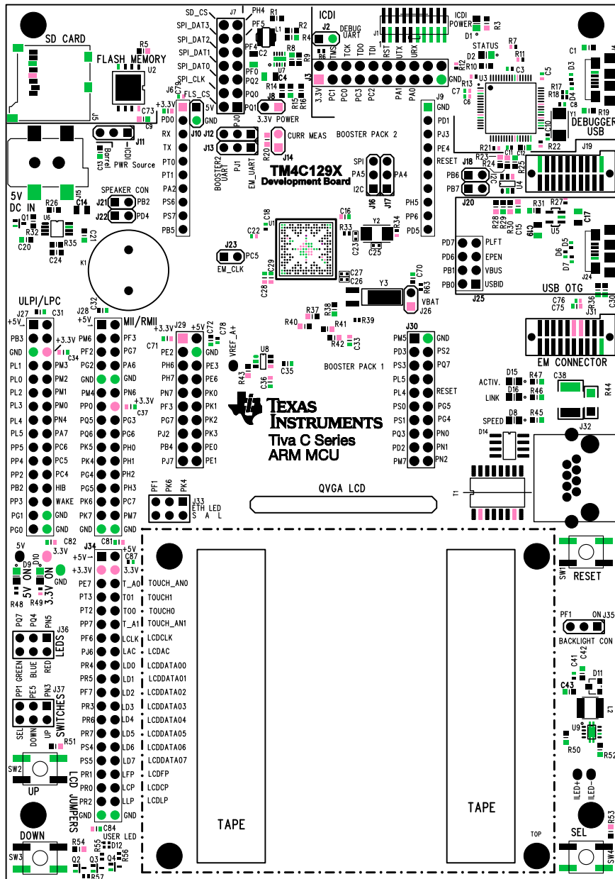
Figure A-1. DK-TM4C129X Component Locations (Top View)
