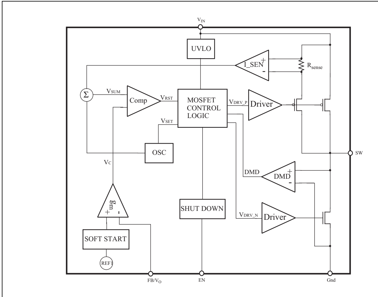
Figure 1. Schematic diagram
