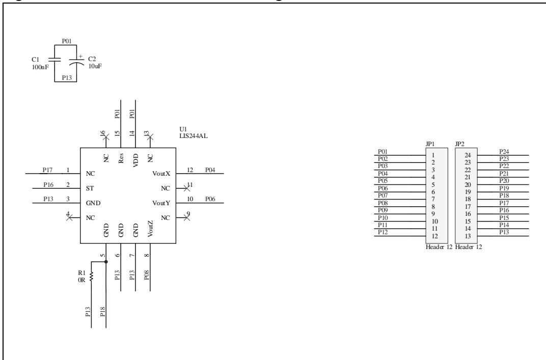
Figure 2. Schematic and connection diagram for the STEVAL-MKI018V1
