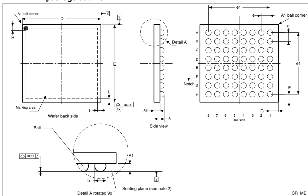
Figure 60. WLCSP, 64-ball 4.466 × 4.395 mm, 0.500 mm pitch, wafer-level chip-scale package outline
