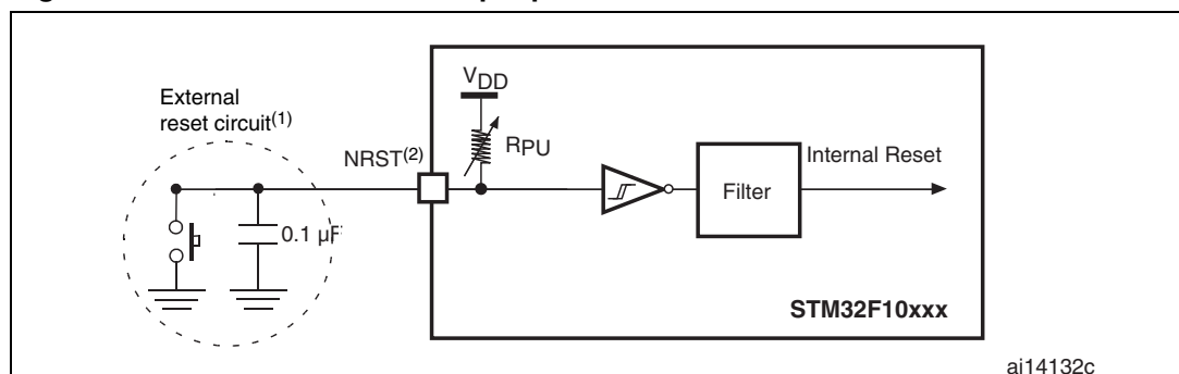
Figure 42. Recommended NRST pin protection
