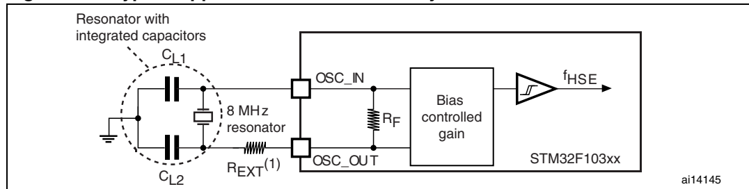
Figure 21. Typical application with an 8 MHz crystal
