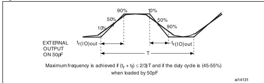
Figure 41. I/O AC characteristics definition
