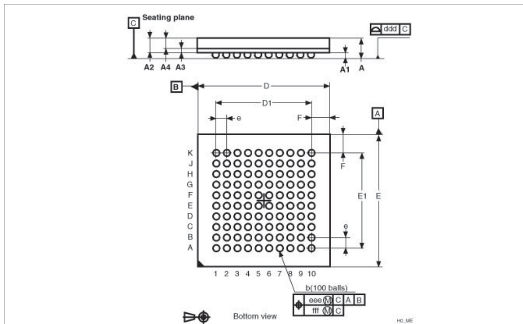
Figure 59. LFBGA100 - 10 x 10 mm low profile fine pitch ball grid array package outline
