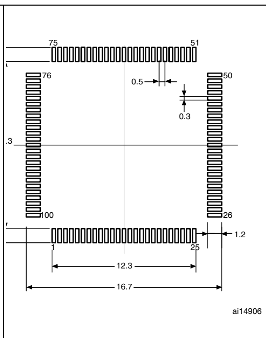
Figure 65. Recommended footprint (1)(2)
