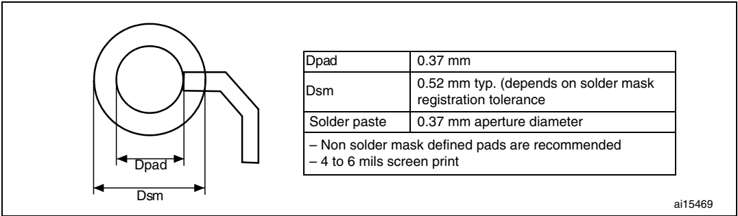
Figure 61. Recommended PCB design rules (0.5 mm pitch BGA)
