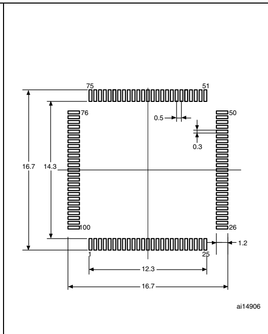
Figure 76. Recommended footprint (1)(2)
