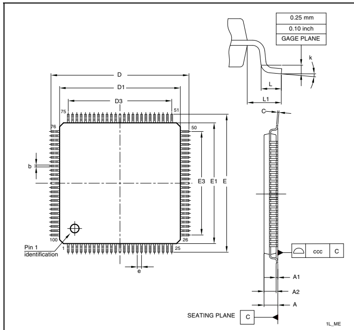
Figure 75. LQFP100, 14 x 14 mm 100-pin low-profile quad flat package outline (1)
