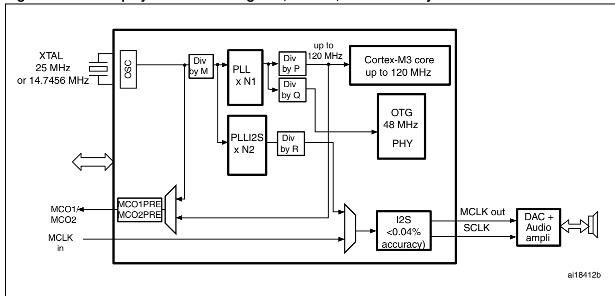
Figure 90. Audio player solution using PLL, PLLI2S, USB and 1 crystal
