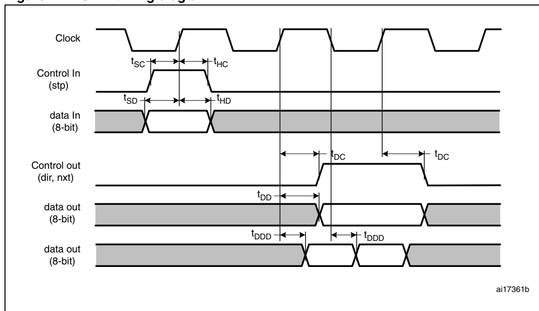
Figure 44. ULPI timing diagram
