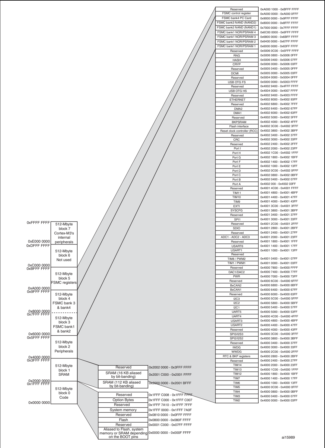
Figure 13. Memory map
