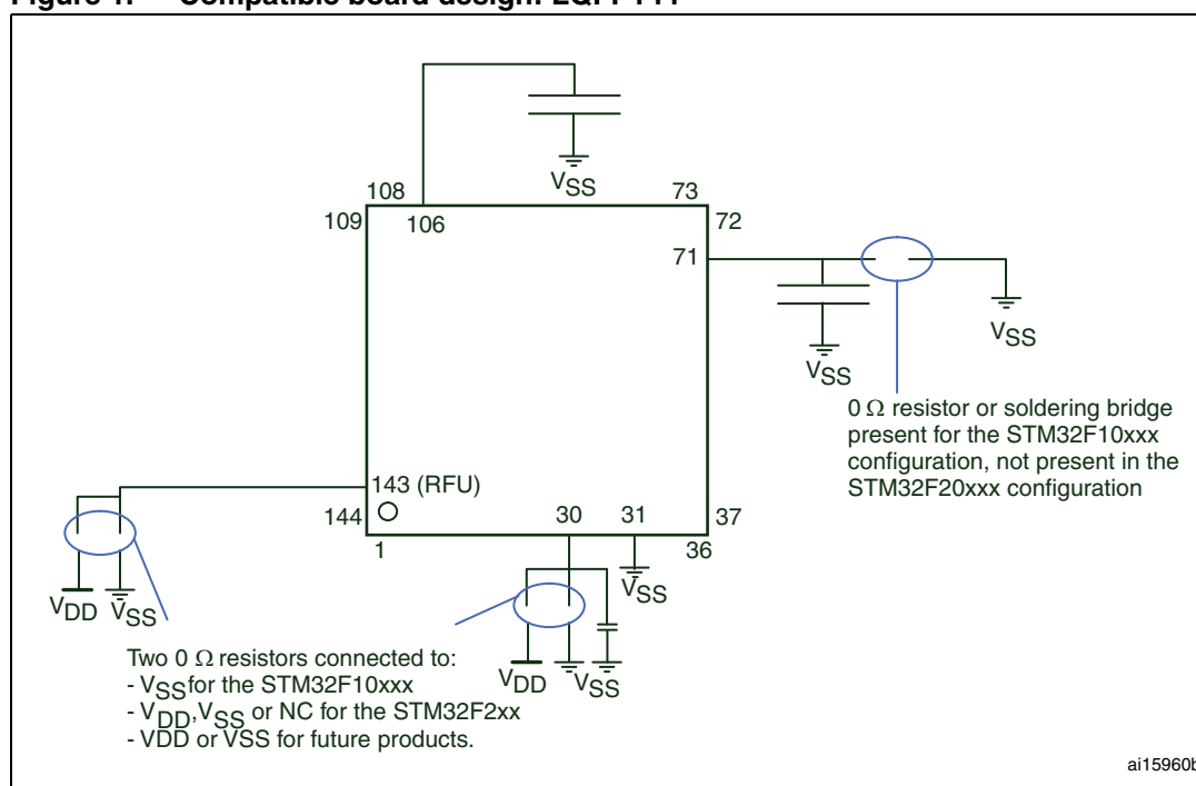
Figure 1. Compatible board design: LQFP144
