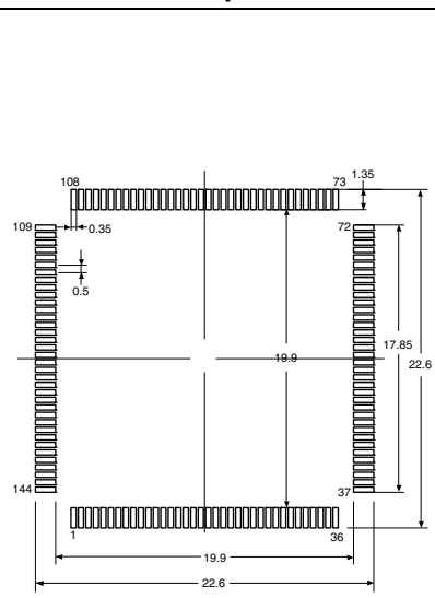
Figure 78. Recommended footprint (1)(2)
