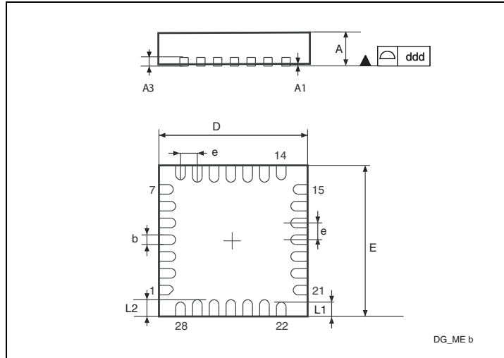
Figure 24. WFQFPN28 – 28-lead very very thin fine pitch quad flat no-lead package outline (4 x 4) (1)
