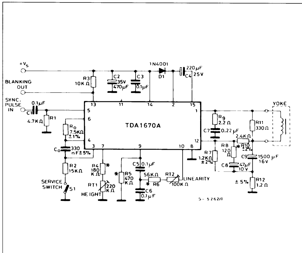
Figure 4 : Application Circuit for 110° TVC set ( R_y = 9.6 \, \Omega ; L_y = 24.6 \, \text{mH} ; I_y = 1.2 \, \text{App} ).
