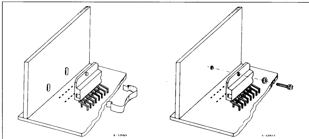
Figure 10 : Mounting Example.
