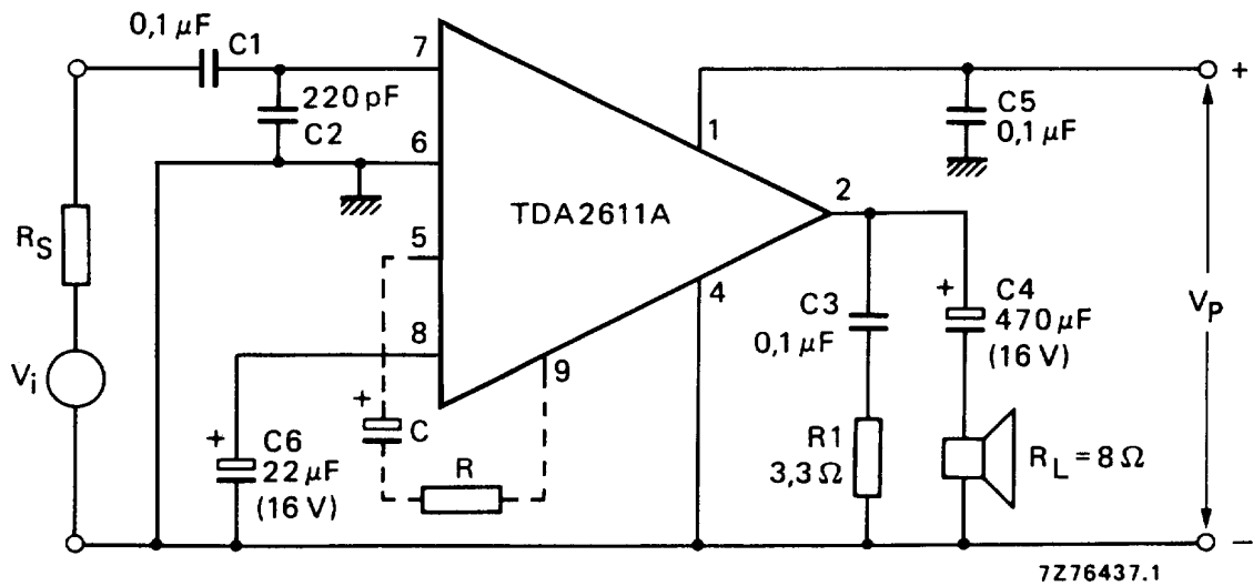
Fig.3 Test circuit; pin 3 not connected.
