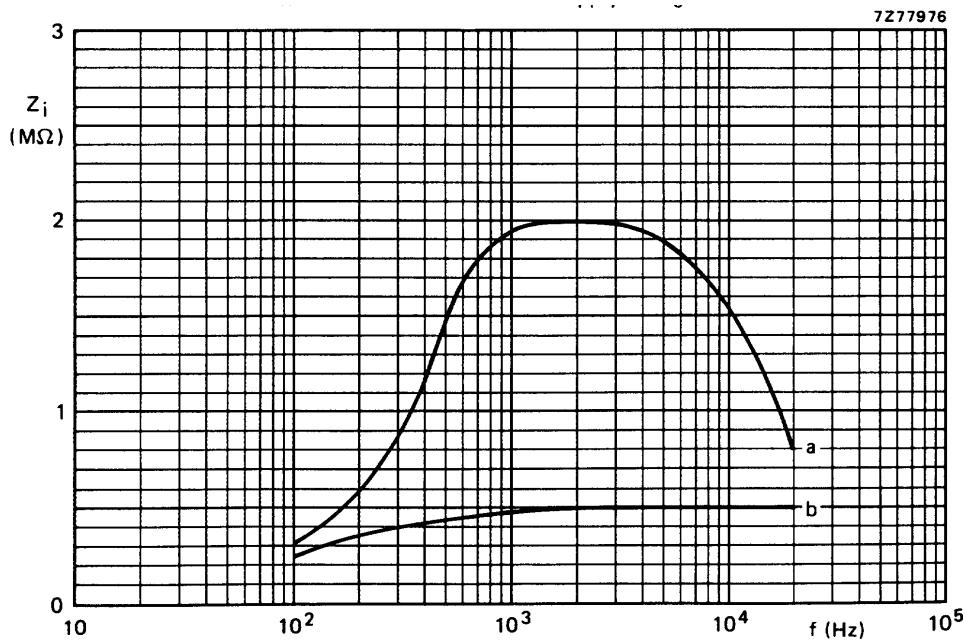
Fig.6 Input impedance as a function of frequency; curve a for C = 1\ \mu\text{F} , R = 0\ \Omega ; curve b for C = 1\ \mu\text{F} , R = 1\ \text{k}\Omega ; circuit of Fig. 3; C_2 = 10\ \text{pF} ; typical values.
