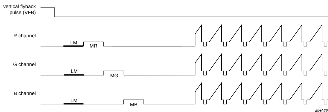
b. Timing controlled by additional vertical flyback pulse (VFB).
