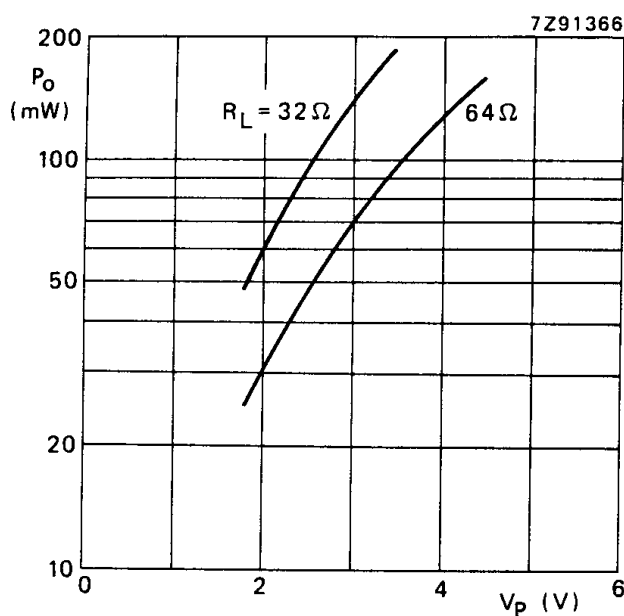
Fig.2 Output power across the load impedance ( R_L ) as a function of supply voltage ( V_p ) in BTL application. Measurements were made at f = 1 kHz; d_{tot} = 10\% ; T_{amb} = 25^\circ\text{C} .
