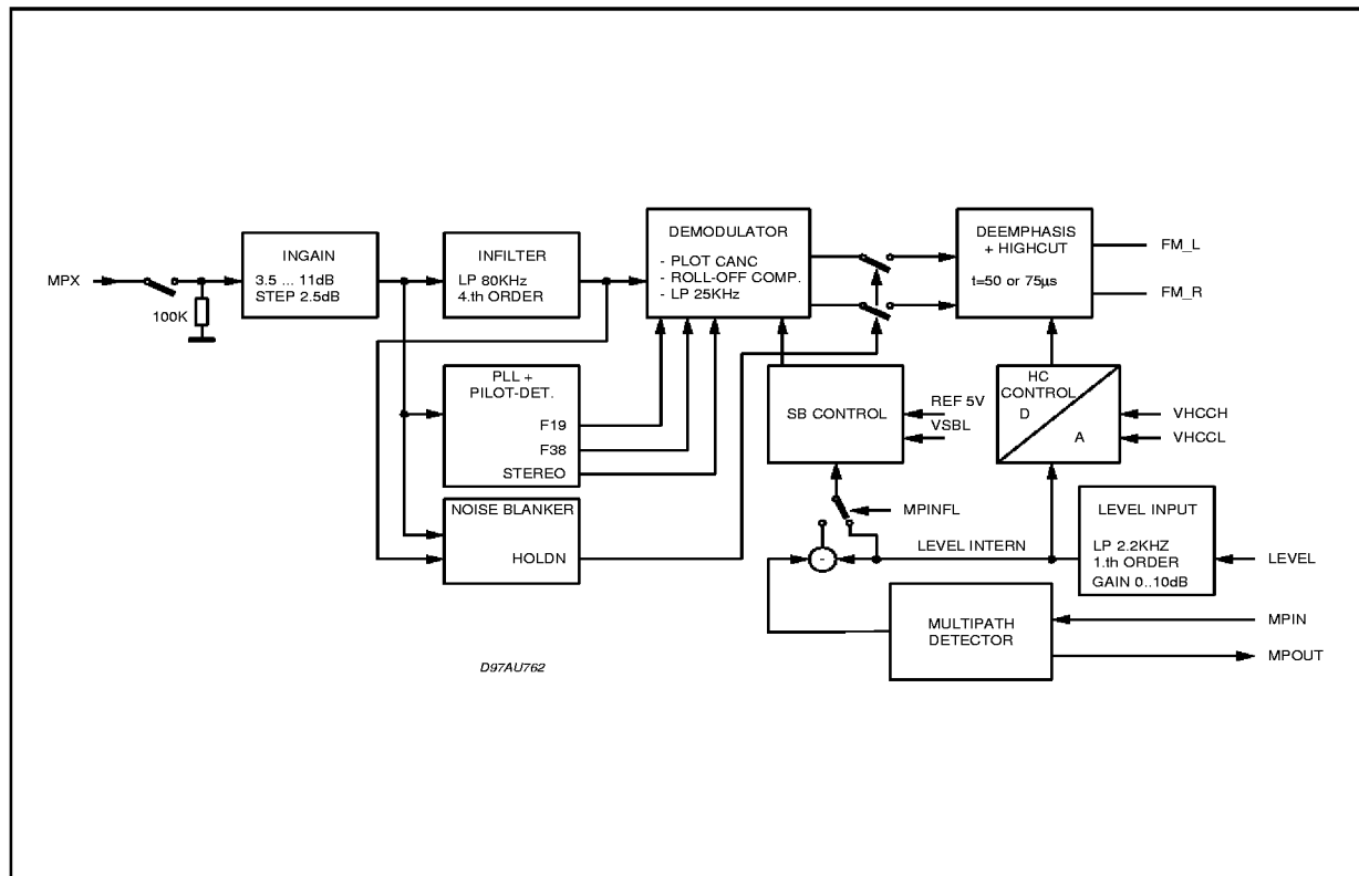
Figure 17. Block diagram of the stereodecoder
