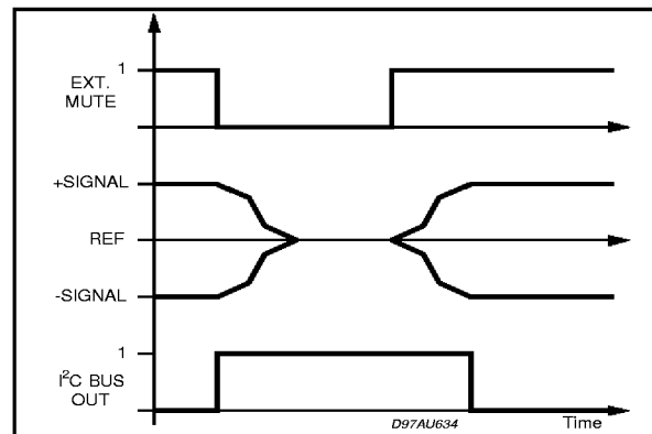
Figure 6. Softmute Timing
