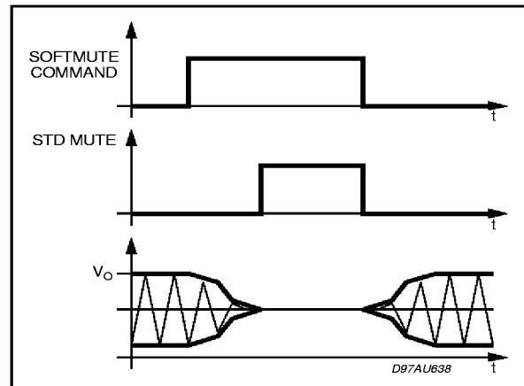
Figure 18. Signals during stereodecoder's softmute
