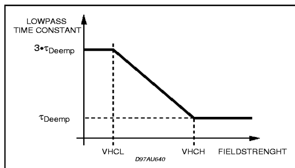
Figure 21. Highcut characteristics
