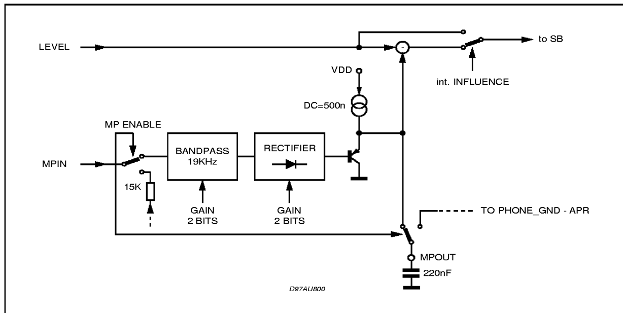
Figure 23. Block diagram of the Multipath Detector
