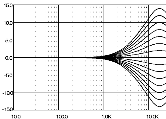
Figure 12. Treble Control @ f_c = 17.5\text{KHz}
