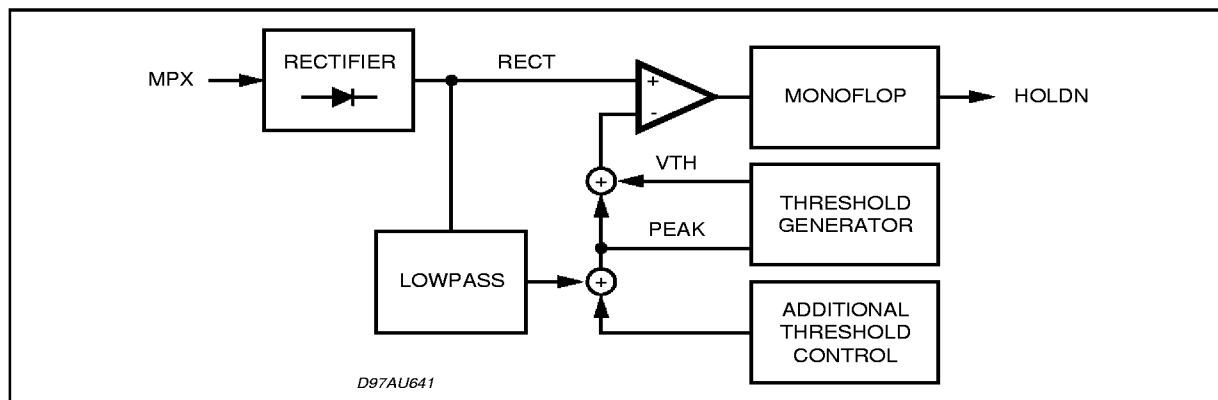
Figure 22. Block diagram of the noiseblanker
