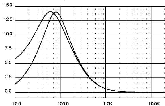
Figure 11. Bass normal and DC Mode @ Gain = 14dB, f_c = 80\text{Hz}
