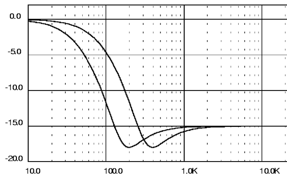
Figure 4. Loudness Center frequency @ Attn. = 15dB (second order)
