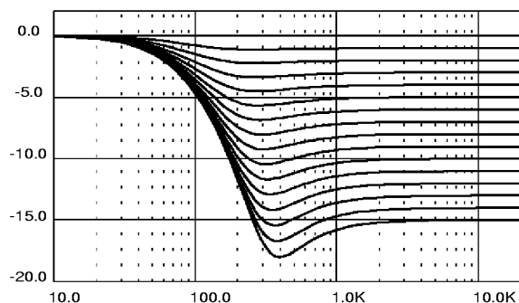
Figure 4. Loudness Center frequency @ Attn. = 15dB (second order)
