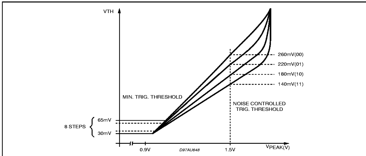
Figure 15. Deviation Controlled Trigger Adjustment
