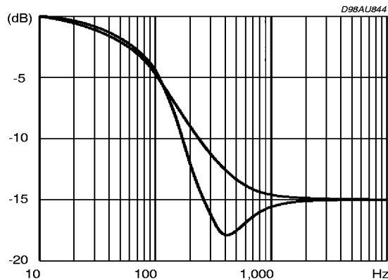
Figure 5. Loudness @ Attn. = 15dB, f_c = 400\text{Hz}
