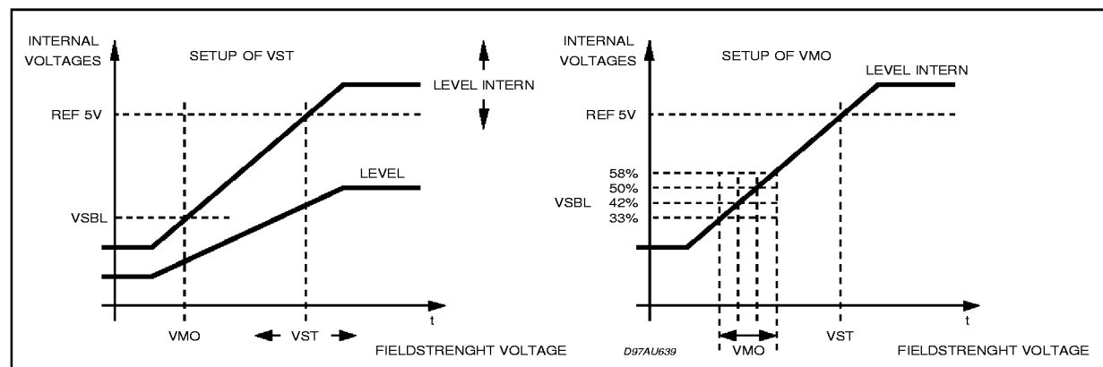
Figure 20. Relation between internal and external LEVEL voltage and setup of Stereoblend
