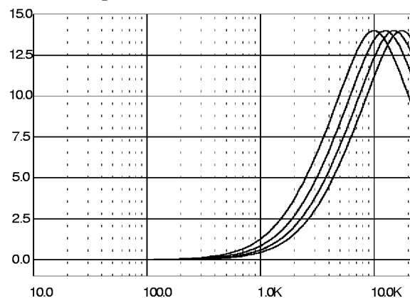
Figure 13. Treble Center Frequencies @ Gain = 14dB
