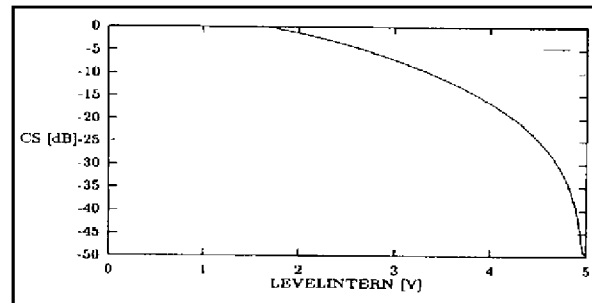
Figure 19. Internal stereoblend characteristics
