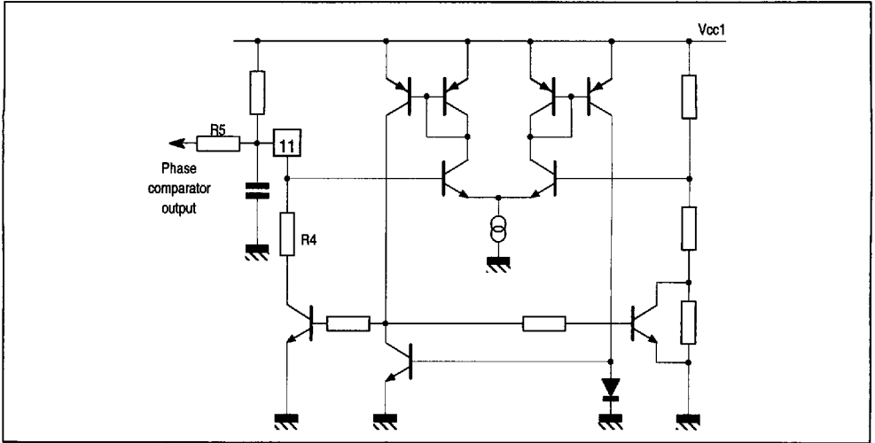
Figure 3 : Line Oscillator
