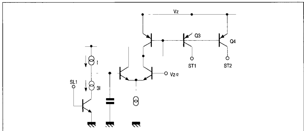
Figure 2 : Frame Separator
