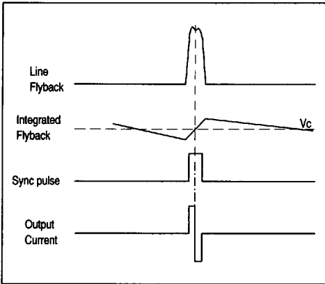
Figure 4 : Phase Comparator
