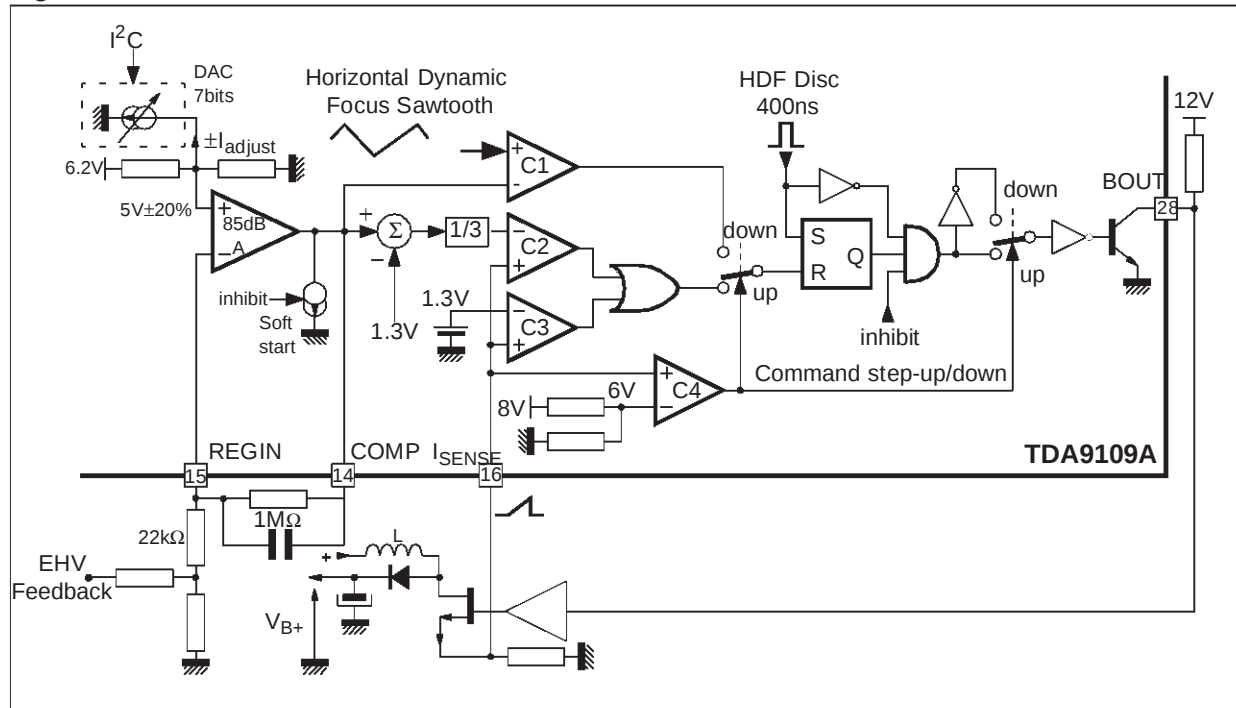
Figure 18. DC/DC Convertor
