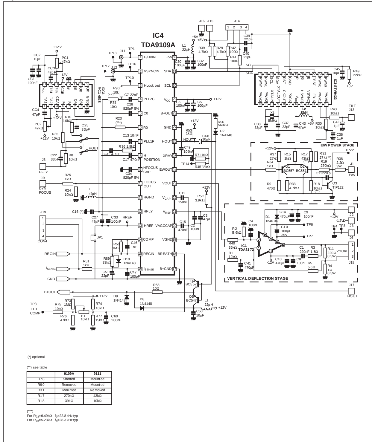
Figure 40. Demonstration Board
