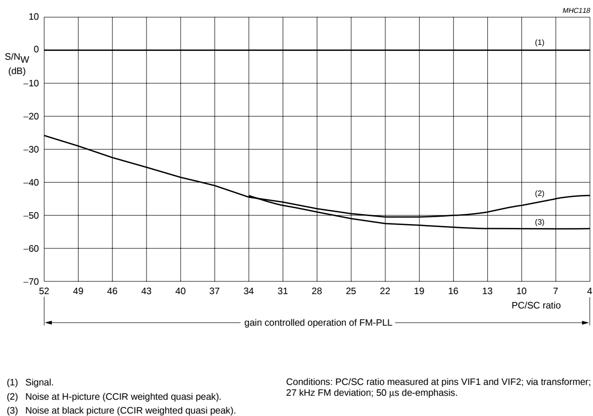
Fig.19 Audio signal-to-noise ratio as a function of picture-to-sound carrier ratio in intercarrier mode.
