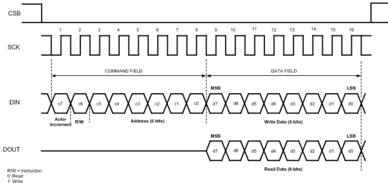
Figure 21. SPI Protocol
