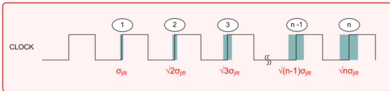
Figure 49. CLOCK Jitter
