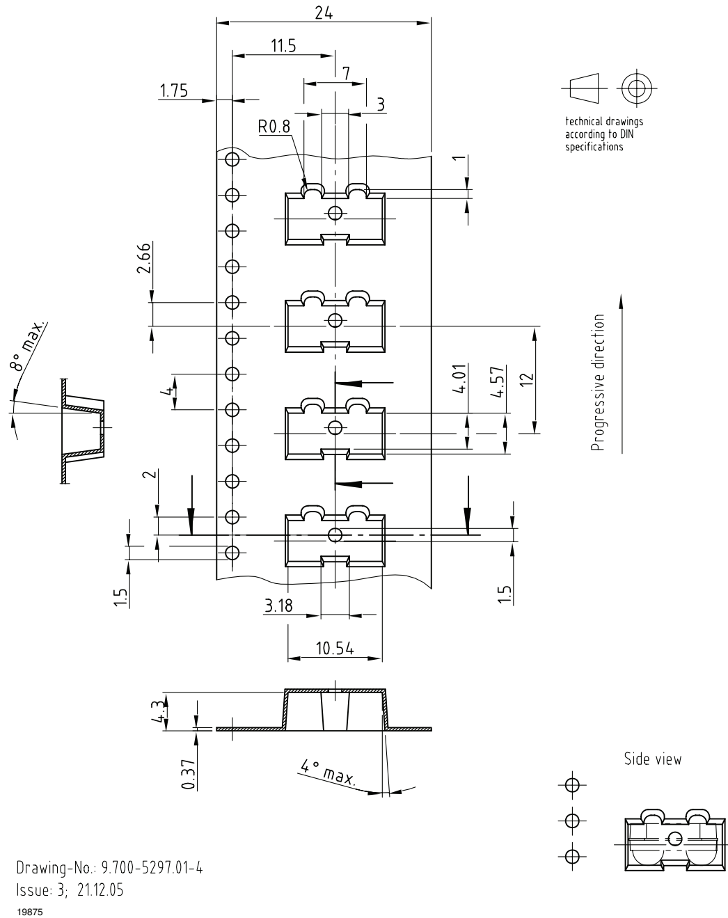
Fig. 11 - Tape Drawing, TFDU4101 for Side View Mounting, Tolerance \pm 0.1 mm
