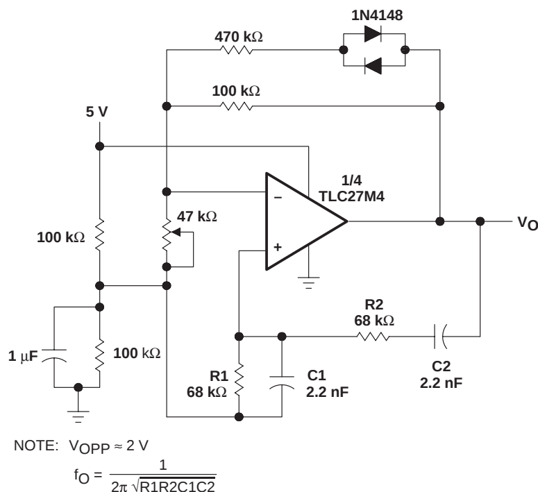
Figure 44. Wien Oscillator
