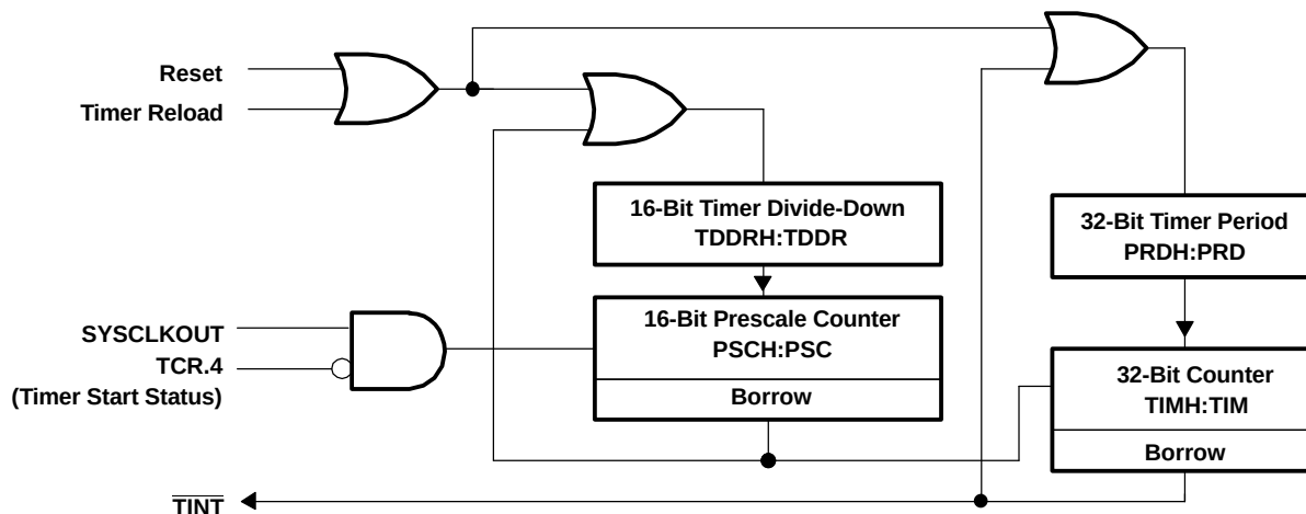
Figure 4-1. CPU-Timers
