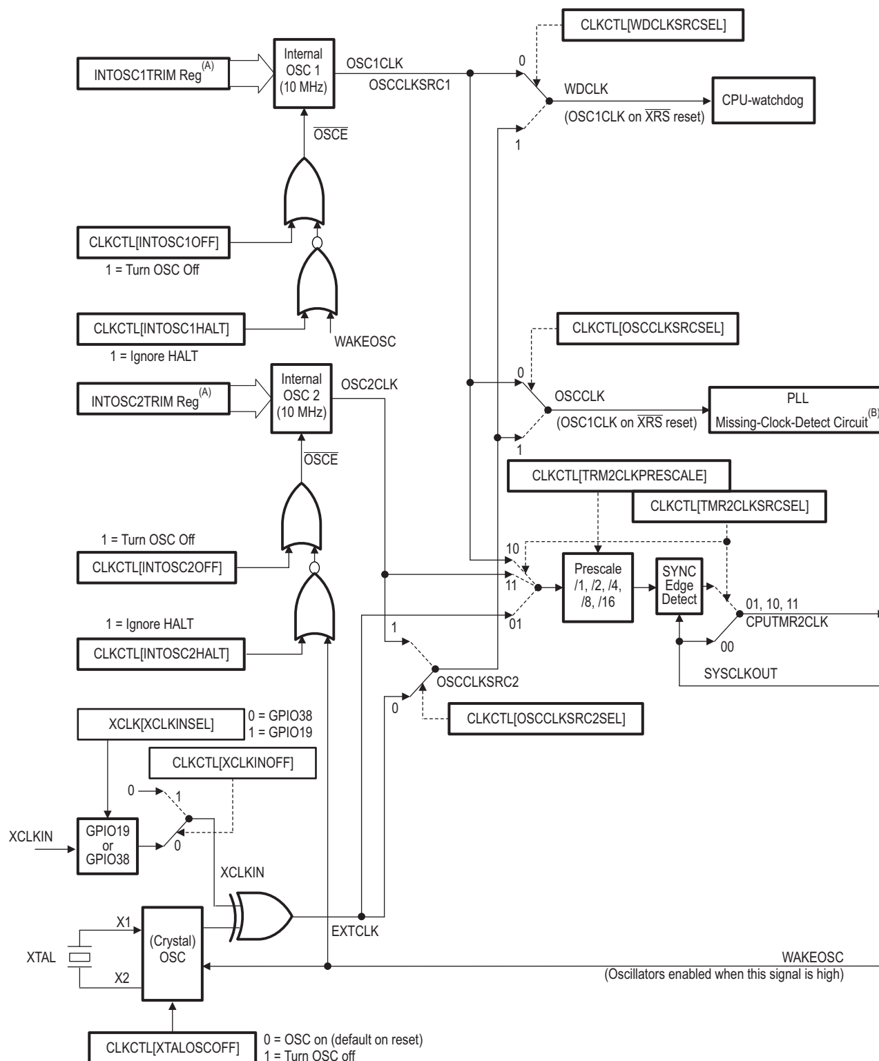
Figure 3-11. Clock Tree
