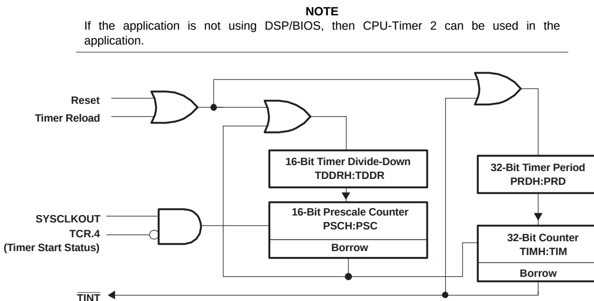
Figure 4-1. CPU-Timers
