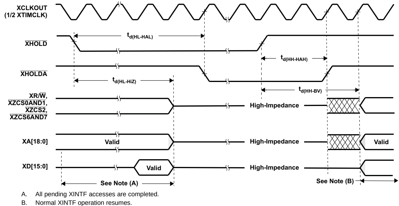
Figure 6-38. \overline{\text{XHOLD}}/\overline{\text{XHOLDA}} Timing Requirements ( \text{XCLKOUT} = 1/2 \text{XTIMCLK} )
