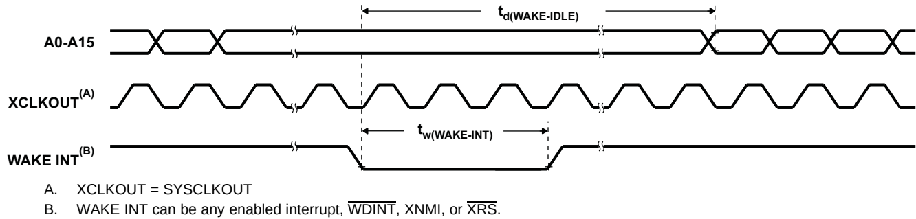
Figure 6-15. IDLE Entry and Exit Timing
