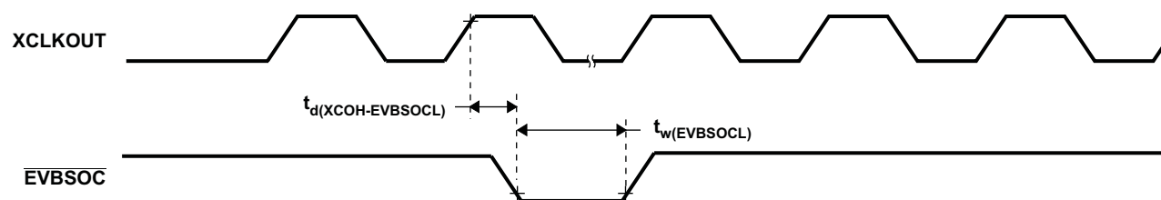
Figure 6-21. \overline{EVBSOC} Timing
