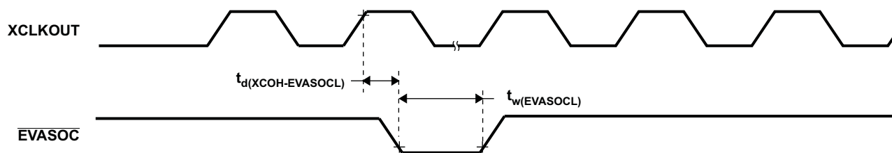
Figure 6-20. \overline{EVASOC} Timing
