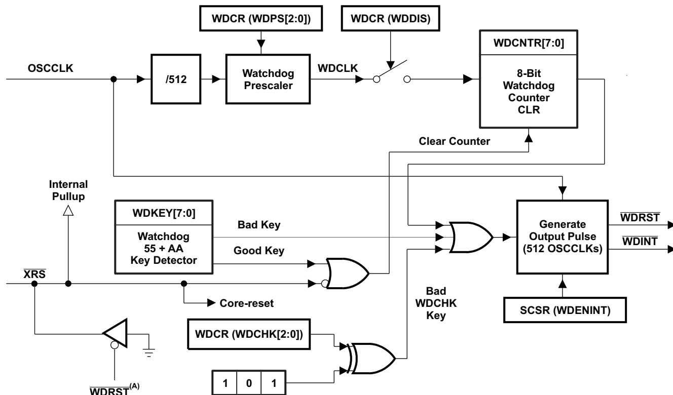
Figure 3-11. Watchdog Module
