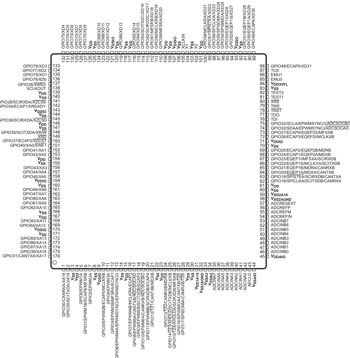
Figure 2-1. F2833x, F2823x 176-Pin PGF/PTP LQFP (Top View)
