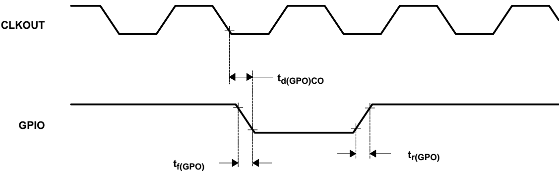
Figure 38. General-Purpose Output Timing
