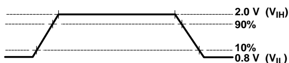
Figure 24. Input Levels
