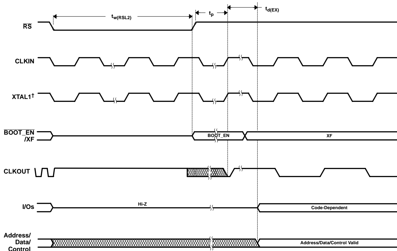
Figure 27. Warm Reset
