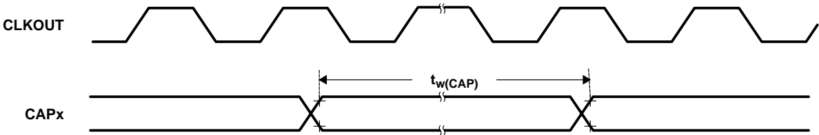
Figure 36. Capture Input and QEP Timing
