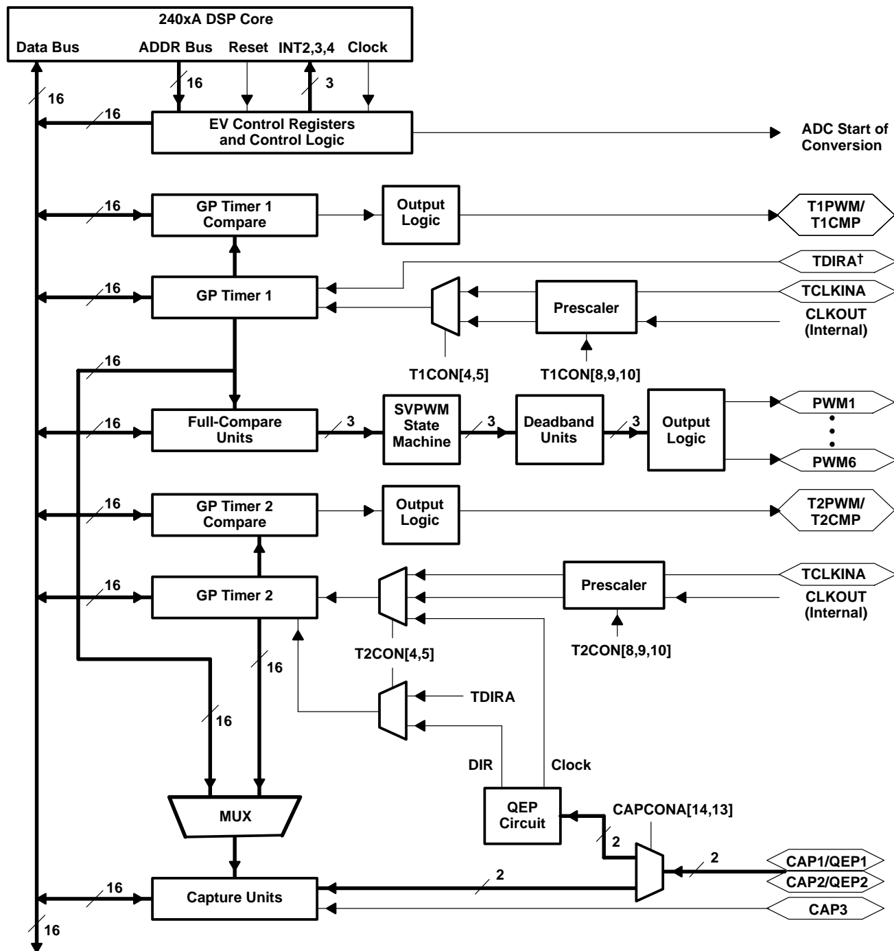
Figure 10. Event Manager A Block Diagram
