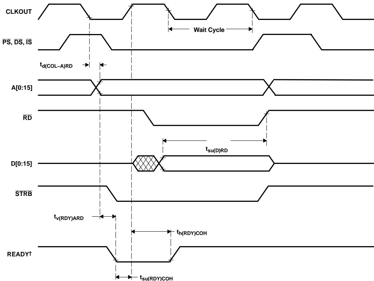
Figure 46. Ready-on-Read Timings
