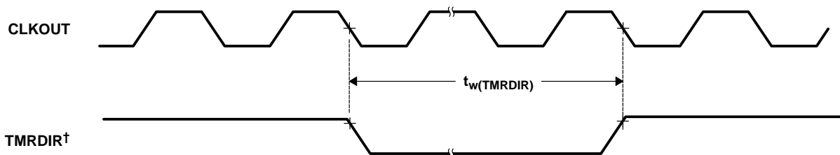
Figure 35. TMRDIR Timing
