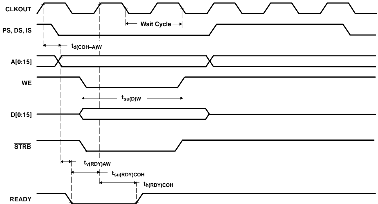
Figure 48. Ready-on-Write Timings
