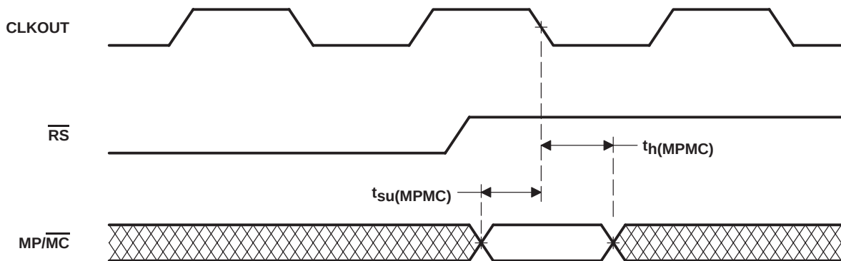
Figure 24. \text{MP}/\overline{\text{MC}} Timing
