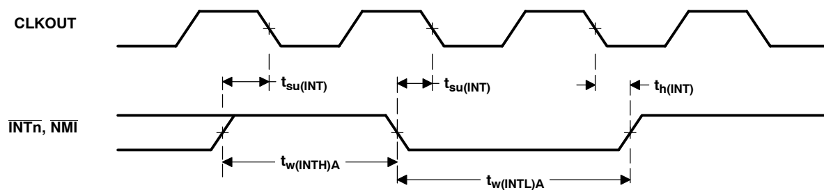
Figure 5-15. Interrupt Timing
