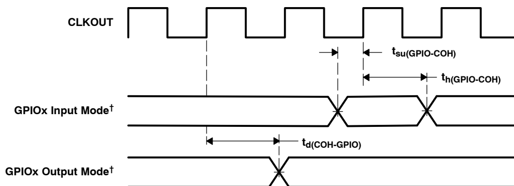
Figure 5–33. GPIOx† Timings
