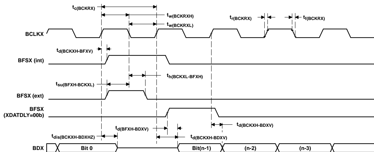
Figure 5-22. McBSP Transmit Timings
