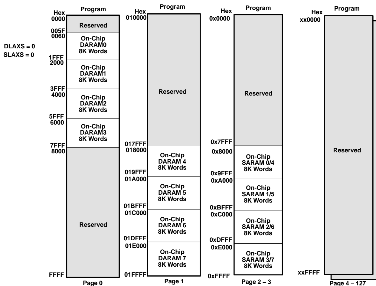
Figure 3-17. On-Chip DMA Memory Map for Program Space (DLAXS = 0 and SLAXS = 0)
