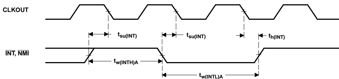
Figure 5-16. Interrupt Timing
