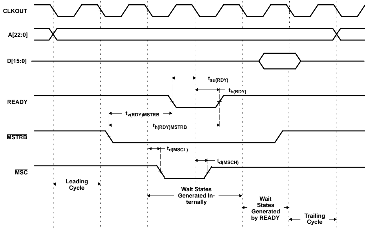
Figure 5-10. Memory Read With Externally Generated Wait States
