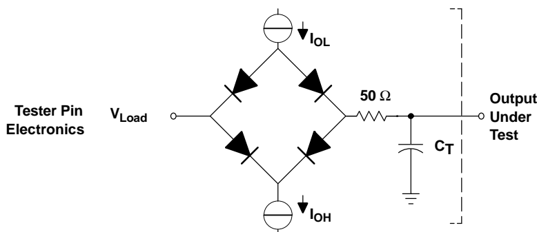
Figure 5-1. 3.3-V Test Load Circuit
