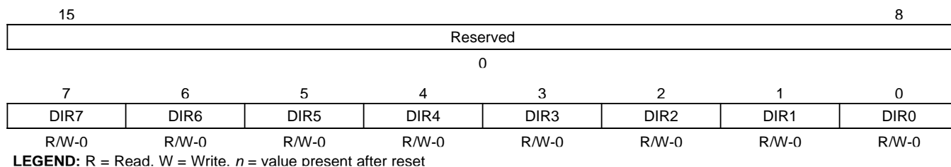
Figure 3-20. General-Purpose I/O Control Register (GPIOCR) [MMR Address 003Ch]
