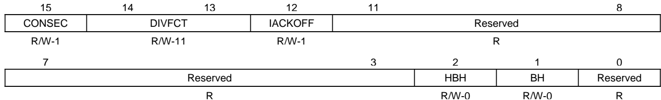
Figure 3-7. Bank-Switching Control Register BSCR)[MMR Address 0029h]
