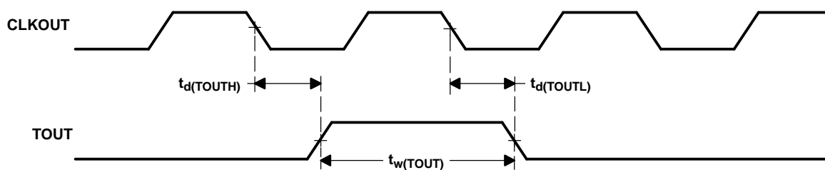
Figure 5-20. TOUT Timing
