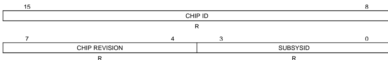
Figure 3-22. Device ID Register (CSIDR) [MMR Address 003Eh]
