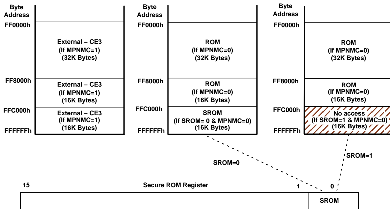
Figure 3–2. Secure ROM
