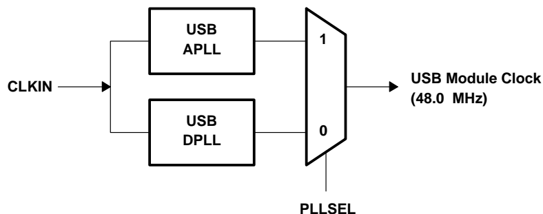
Figure 3-18. USB Clock Generation
