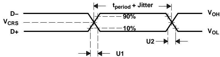
Figure 5–41. USB Timings
