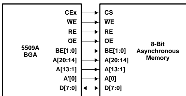
Figure 3–8. Parallel Port (EMIF) Signal Interface
