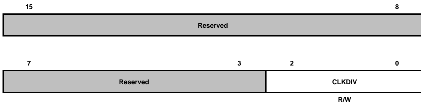
Figure 3-17. System Register Bit Locations
