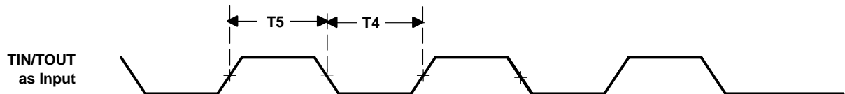
Figure 5–22. TIN/TOUT Timings When Configured as Inputs
