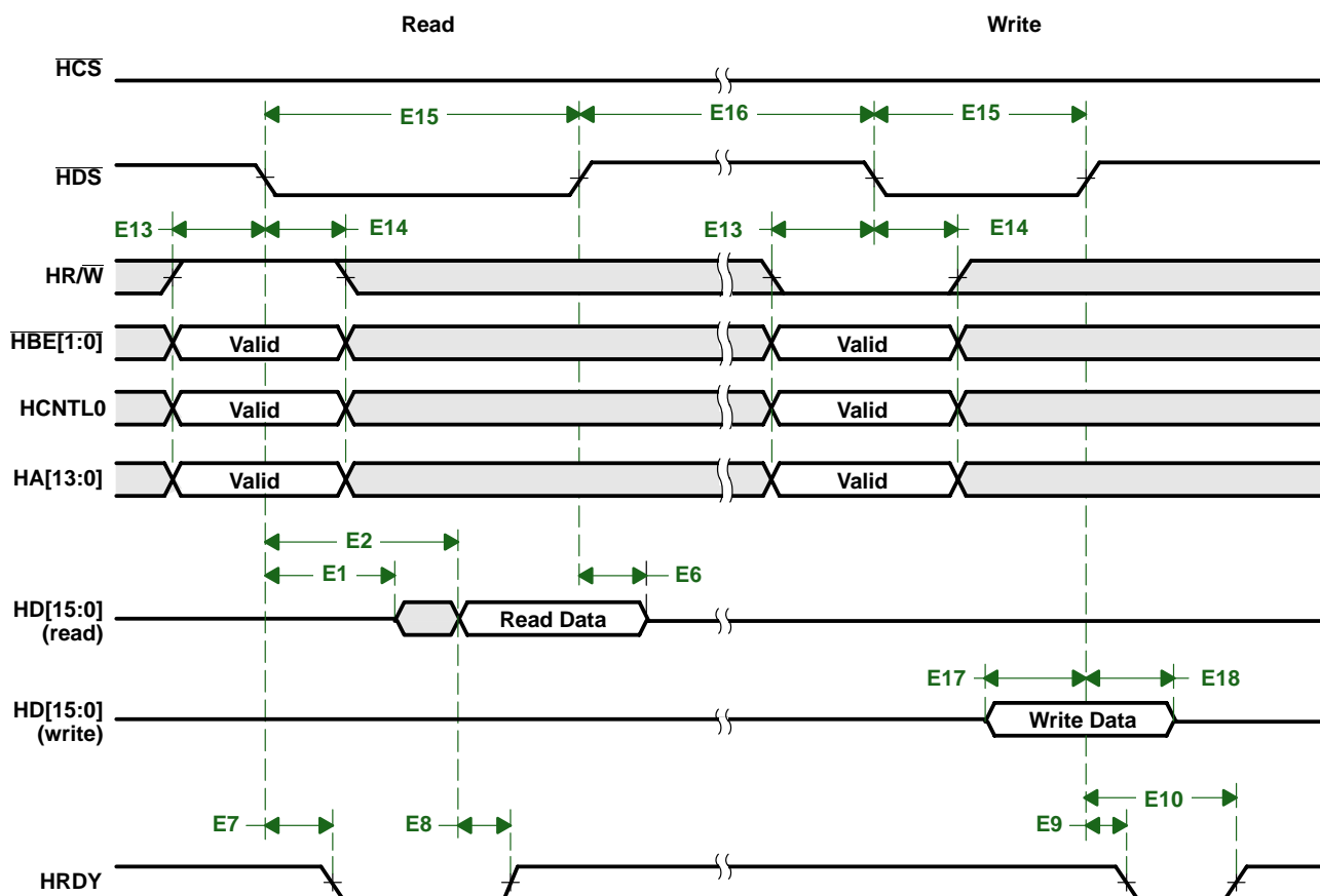
Figure 5–31. HINT Timings
