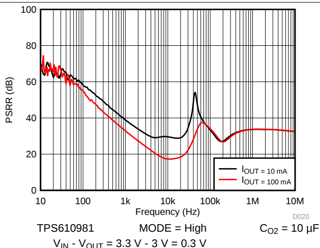
Figure 36. LDO PSRR vs Frequency
