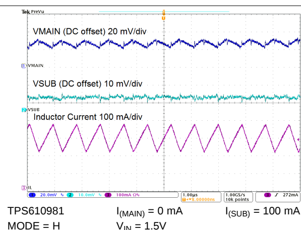
Figure 50. Switching Waveforms
