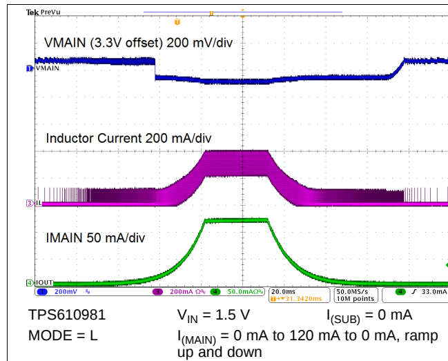
Figure 57. Load Regulation
