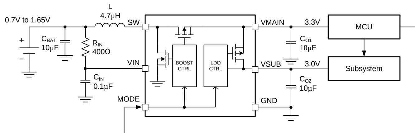
Figure 43. Typical Application of TPS610981 to Power Low Power System
