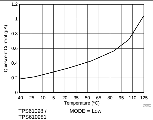
Figure 2. I_Q into VMAIN Pin at Low Power Mode vs Temperature
