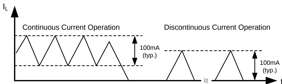
Figure 39. Hysteretic Current Operation
