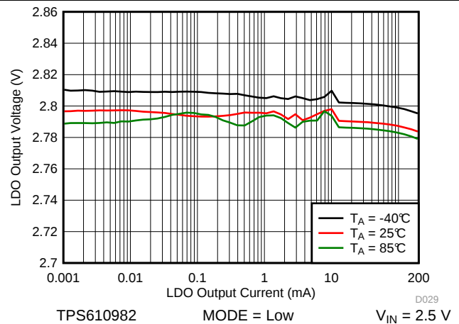
Figure 28. LDO Load Regulation at Low Power Mode
