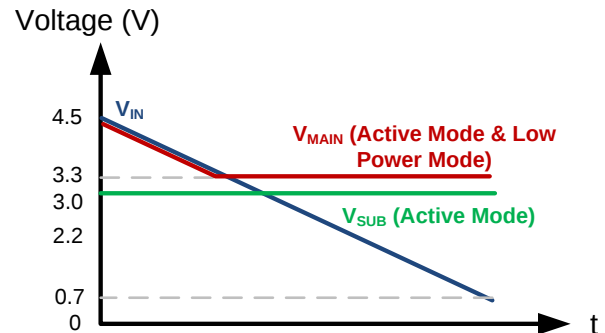
Figure 42. TPS610981 Output under Different Input Voltages
