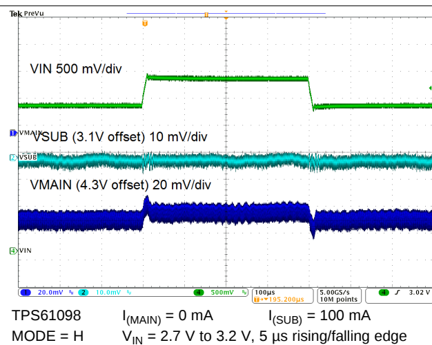
Figure 69. Line Transient Response
