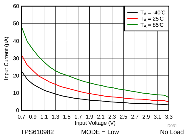
Figure 33. No Load Input Current vs Input Voltage at Low Power Mode
