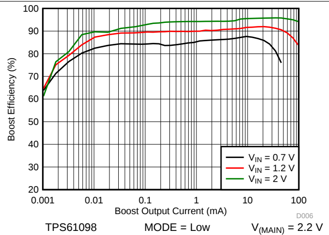
Figure 14. Boost Efficiency vs Output Current at Low Power Mode
