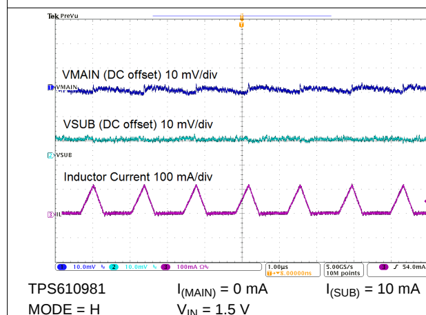
Figure 49. Switching Waveforms
