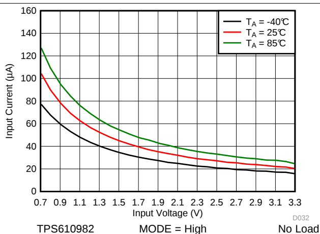
Figure 34. No Load Input Current vs Input Voltage at Active Mode
