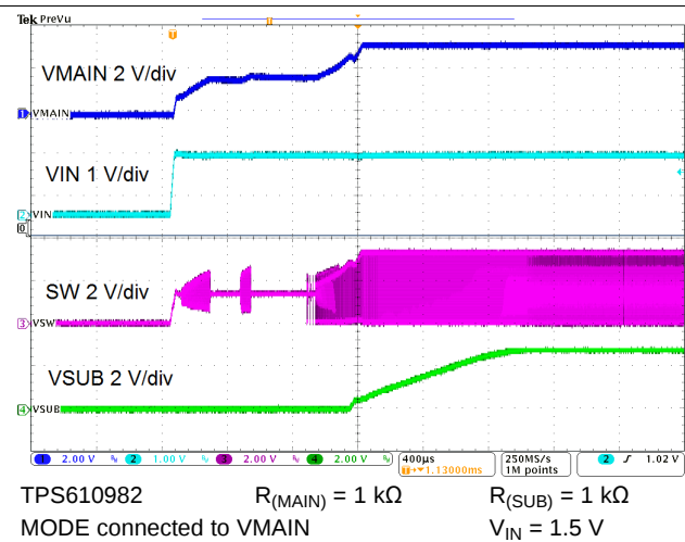
Figure 77. Startup
