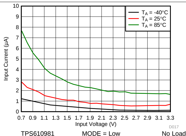
Figure 31. No Load Input Current vs Input Voltage at Low Power Mode
