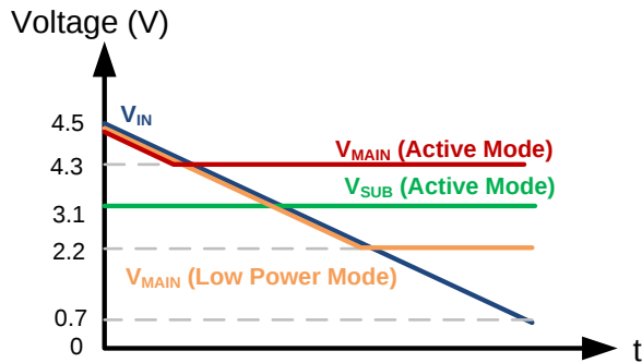
Figure 41. TPS61098 Output under Different Input Voltages
