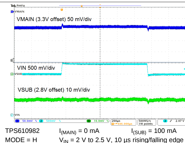
Figure 71. Line Transient Response
