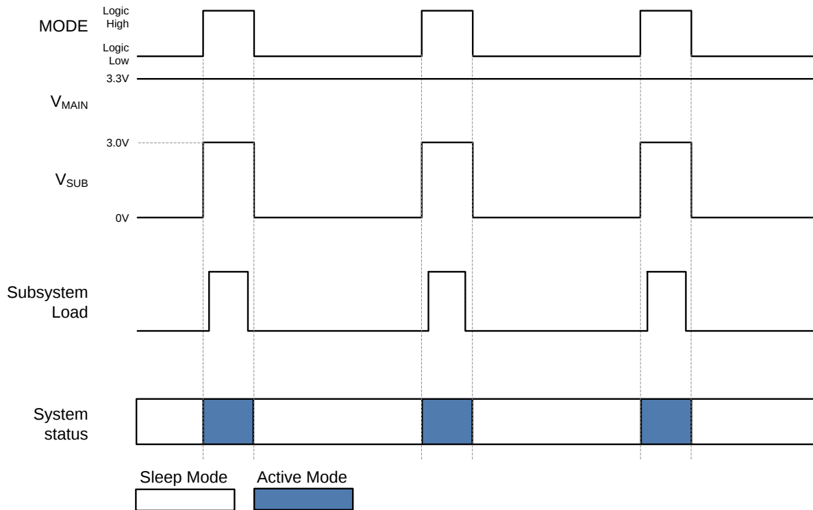
Figure 44. System Control Sequence
