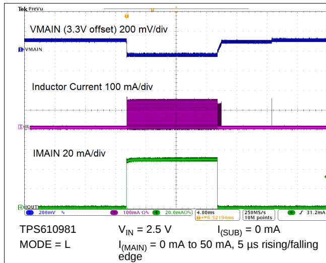
Figure 51. Load Transient Response
