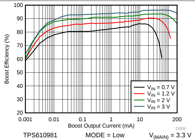
Figure 16. Boost Efficiency vs Output Current at Low Power Mode
