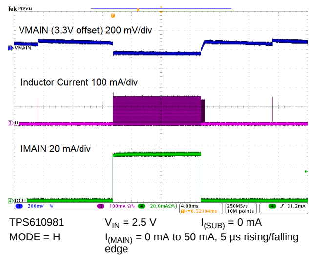
Figure 52. Load Transient Response
