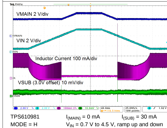
Figure 59. Line Regulation
