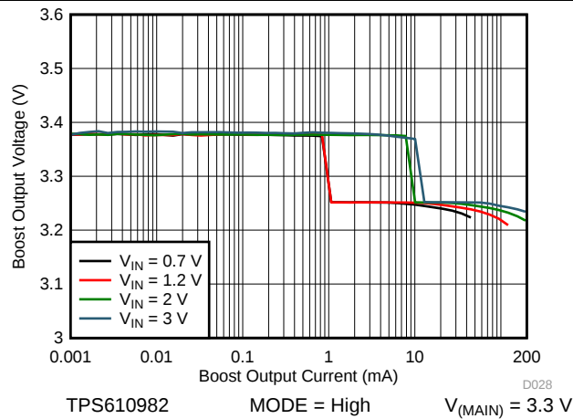
Figure 25. Boost Load Regulation at Active Mode
