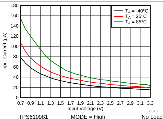
Figure 32. No Load Input Current vs Input Voltage at Active Mode
