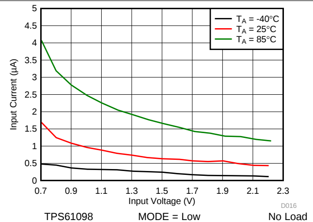
Figure 30. No Load Input Current vs Input Voltage at Low Power Mode
