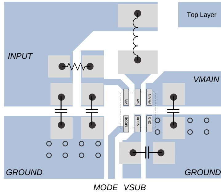
Figure 78. Layout
