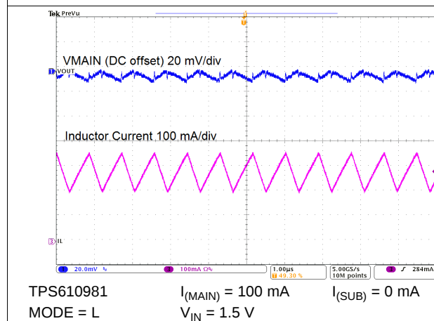
Figure 47. Switching Waveforms
