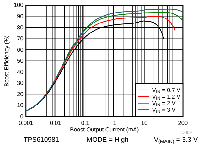
Figure 17. Boost Efficiency vs Output Current at Active Mode
