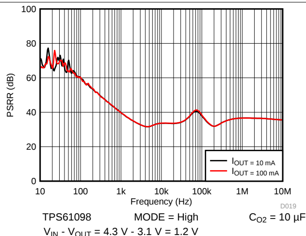
Figure 35. LDO PSRR vs Frequency
