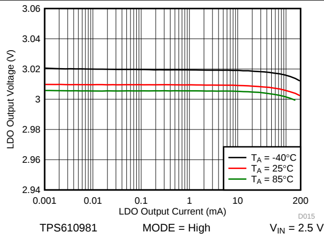
Figure 27. LDO Load Regulation
