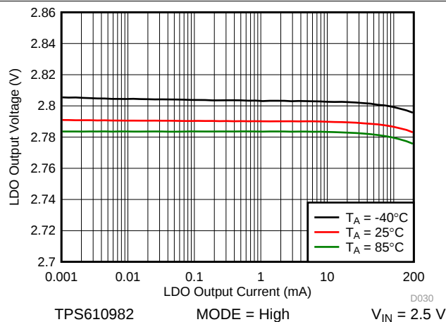
Figure 29. LDO Load Regulation at Active Mode
