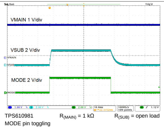
Figure 60. Mode Toggling
