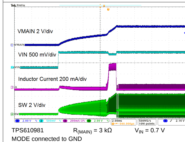
Figure 61. Startup
