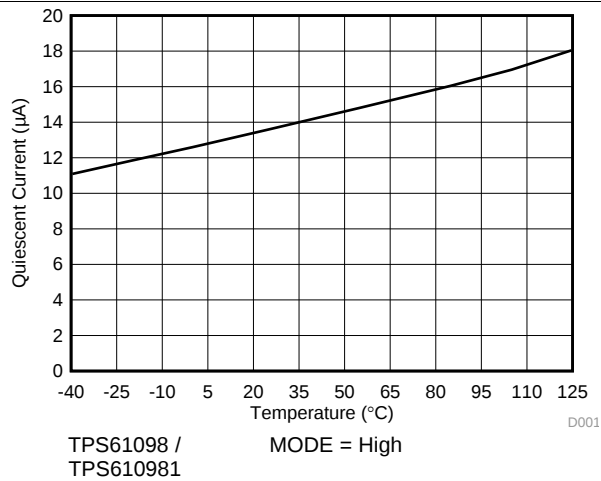
Figure 1. I_Q into VMAIN Pin at Active Mode vs Temperature
