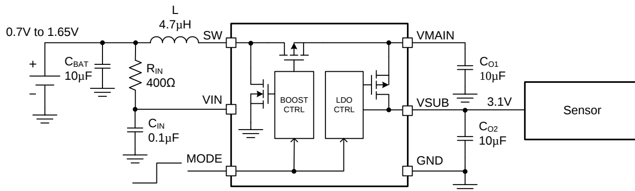
Figure 67. Typical Application of TPS61098 VSUB to Power the System in Active Mode
