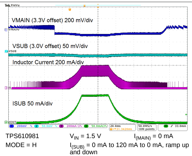
Figure 58. Load Regulation
