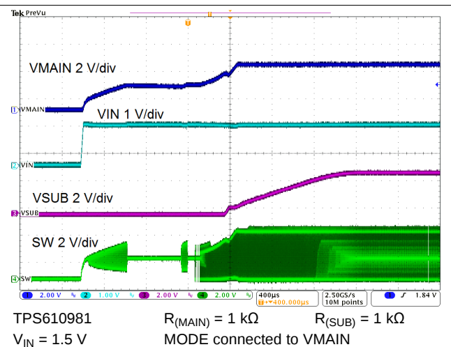
Figure 62. Startup
