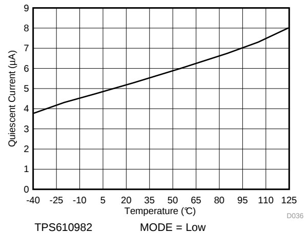
Figure 4. I_Q into VMAIN Pin at Low Power Mode vs Temperature
