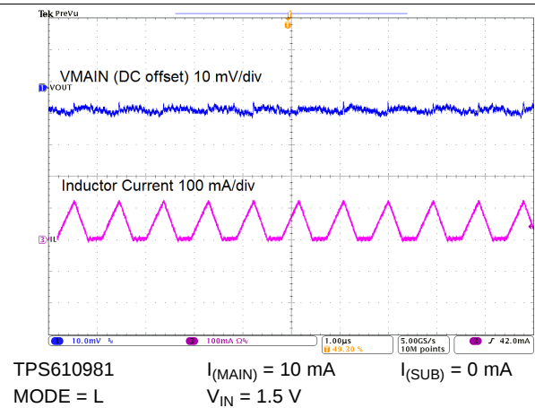
Figure 46. Switching Waveforms
