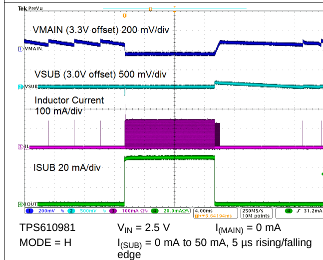
Figure 53. LDO Load Transient Response
