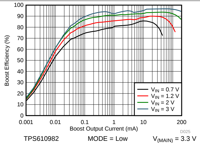
Figure 18. Boost Efficiency vs Output Current at Low Power Mode
