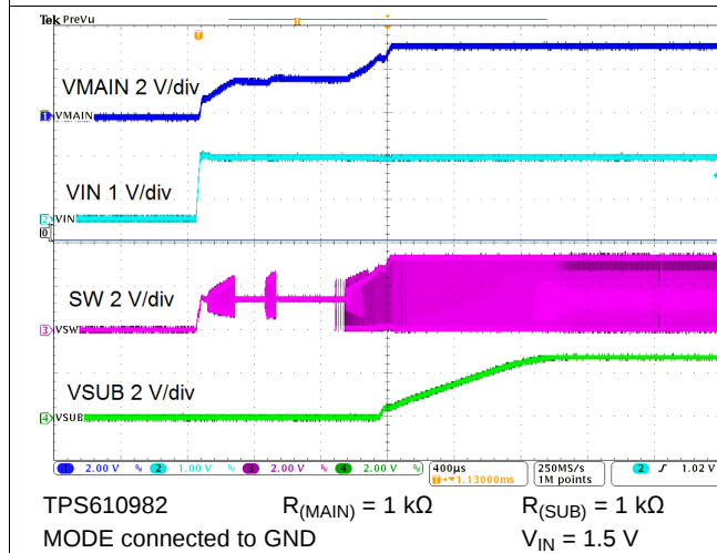
Figure 76. Startup
