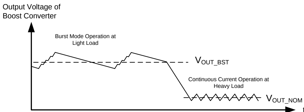
Figure 40. Burst Mode Operation
