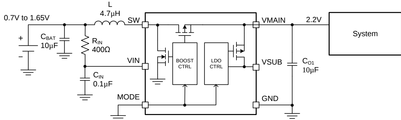
Figure 63. Typical Application of TPS61098 VMAIN to Power the System in Low Power Mode
