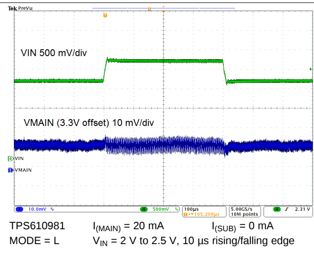
Figure 54. Line Transient Response
