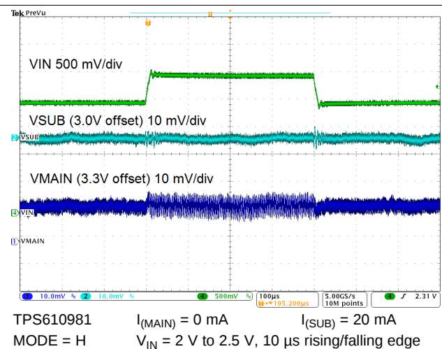
Figure 56. Line Transient Response
