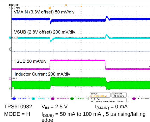
Figure 73. LDO Load Transient Response
