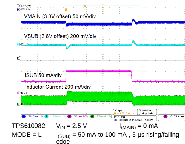
Figure 72. LDO Load Transient Response
