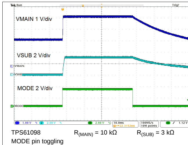
Figure 74. MODE Toggling
