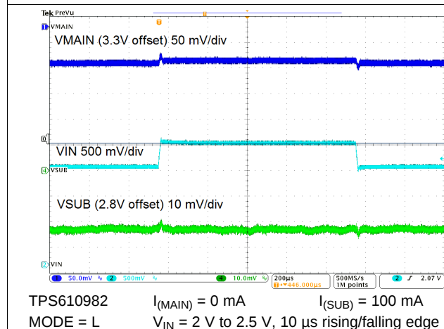
Figure 70. Line Transient Response
