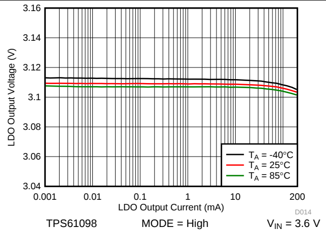
Figure 26. LDO Load Regulation
