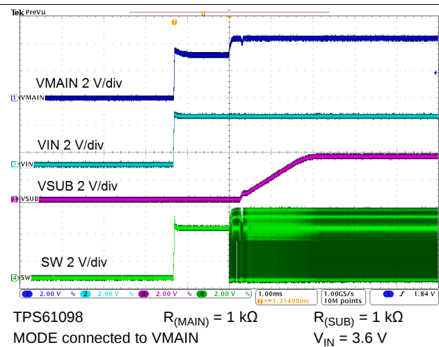
Figure 75. Startup
