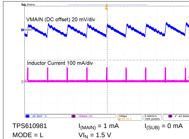
Figure 45. Switching Waveforms
