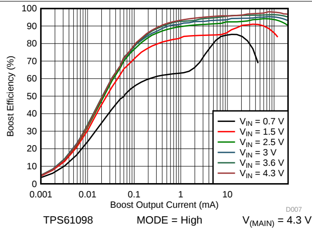
Figure 15. Boost Efficiency vs Output Current at Active Mode
