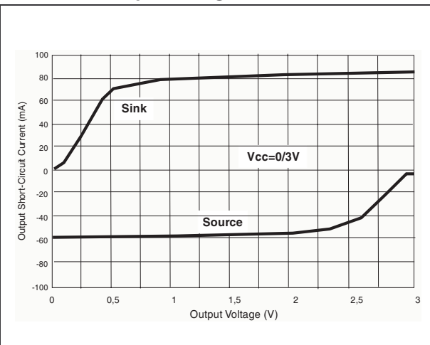
Figure 2. Output short circuit current vs. output voltage
