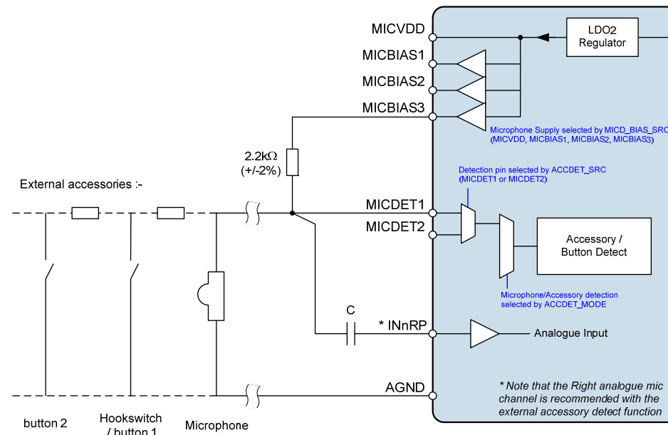
Figure 64 Microphone and Accessory Detect Interface
