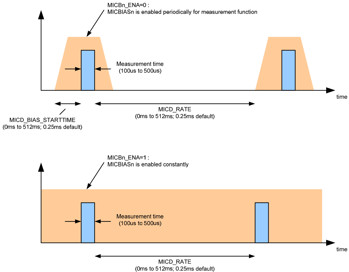
Figure 65 Microphone and Accessory Detect Timing
