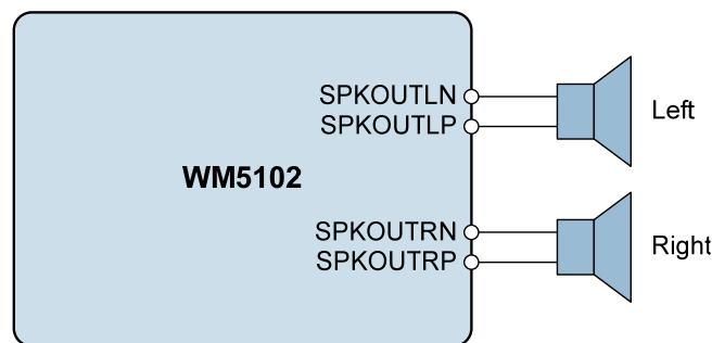
Figure 58 Speaker Connection
