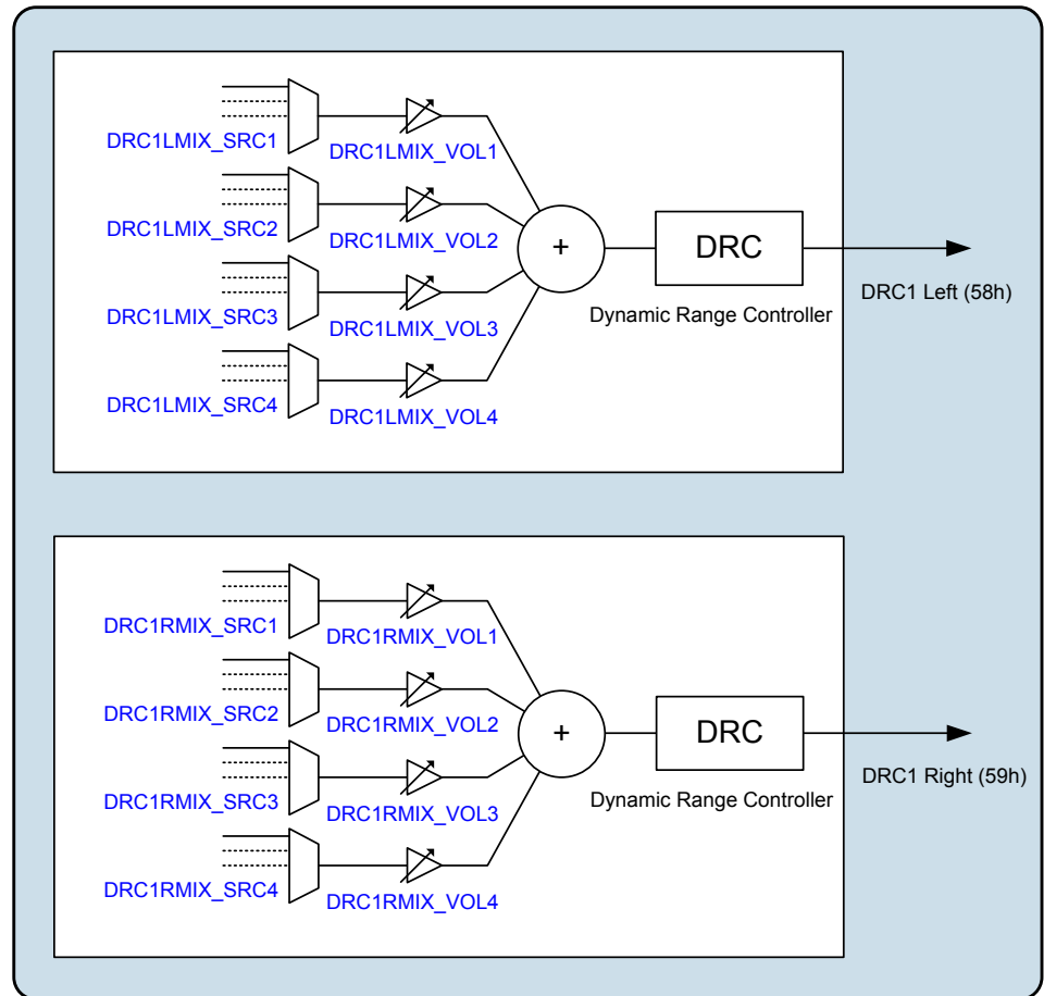
Figure 30 Dynamic Range Control (DRC) Block
