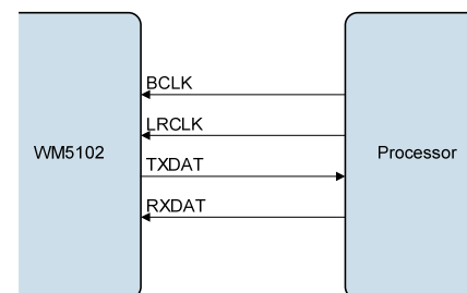
Figure 44 Slave Mode
