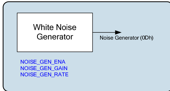
Figure 35 Digital Core Noise Generator
