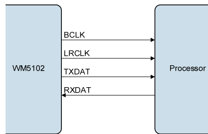
Figure 43 Master Mode
