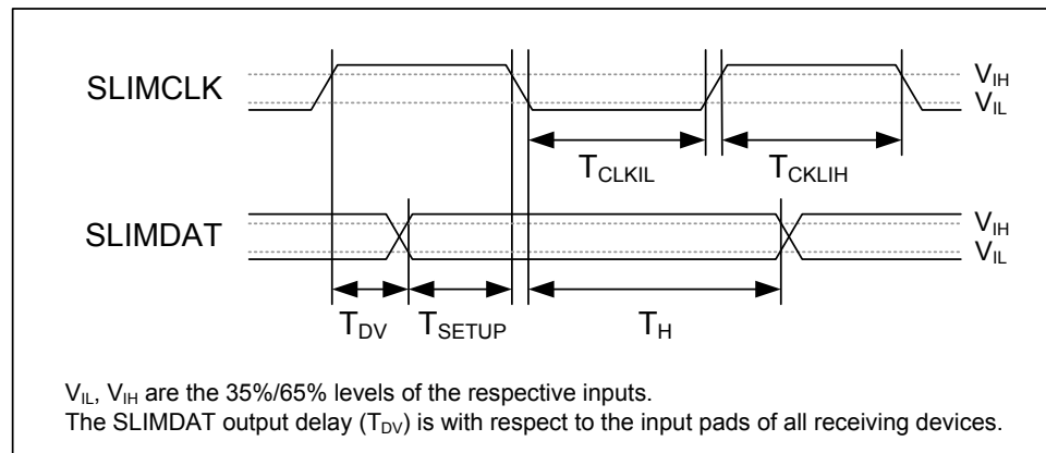
Figure 12 SLIMbus Interface Timing
