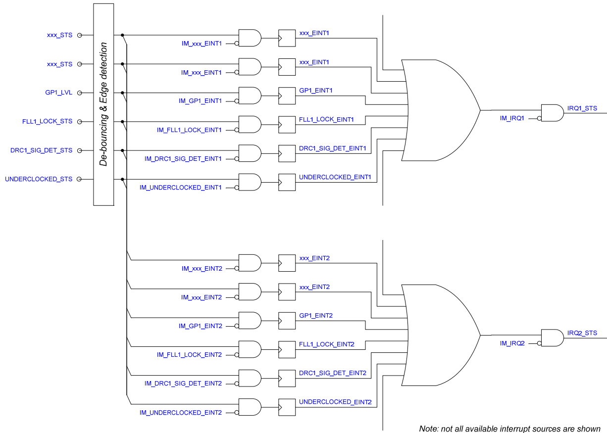
Figure 67 Interrupt Controller
