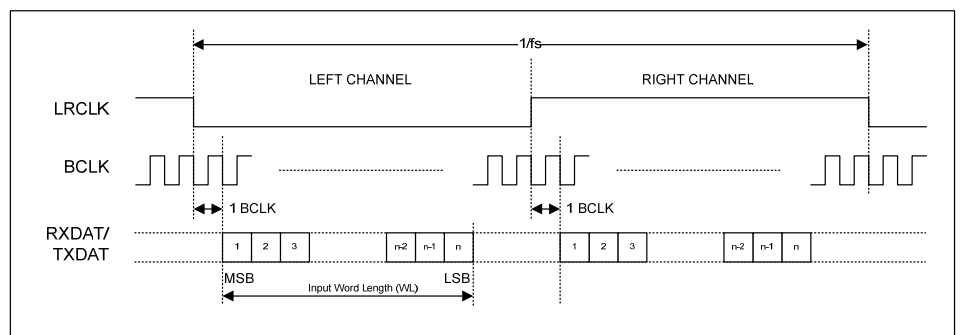
Figure 47 I2S Data Format (assuming n-bit word length)
