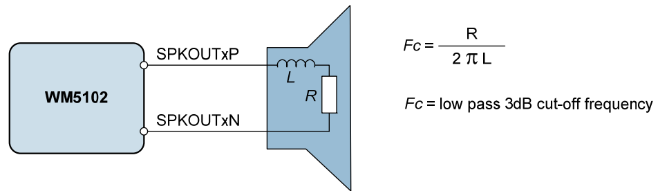
Figure 90 Speaker Equivalent Circuit for Filterless Operation
