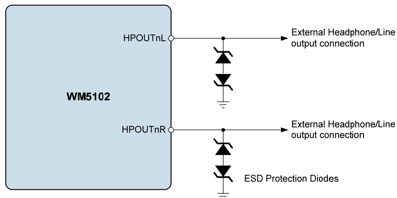
Figure 87 ESD Diode Configuration for External Output Connections
