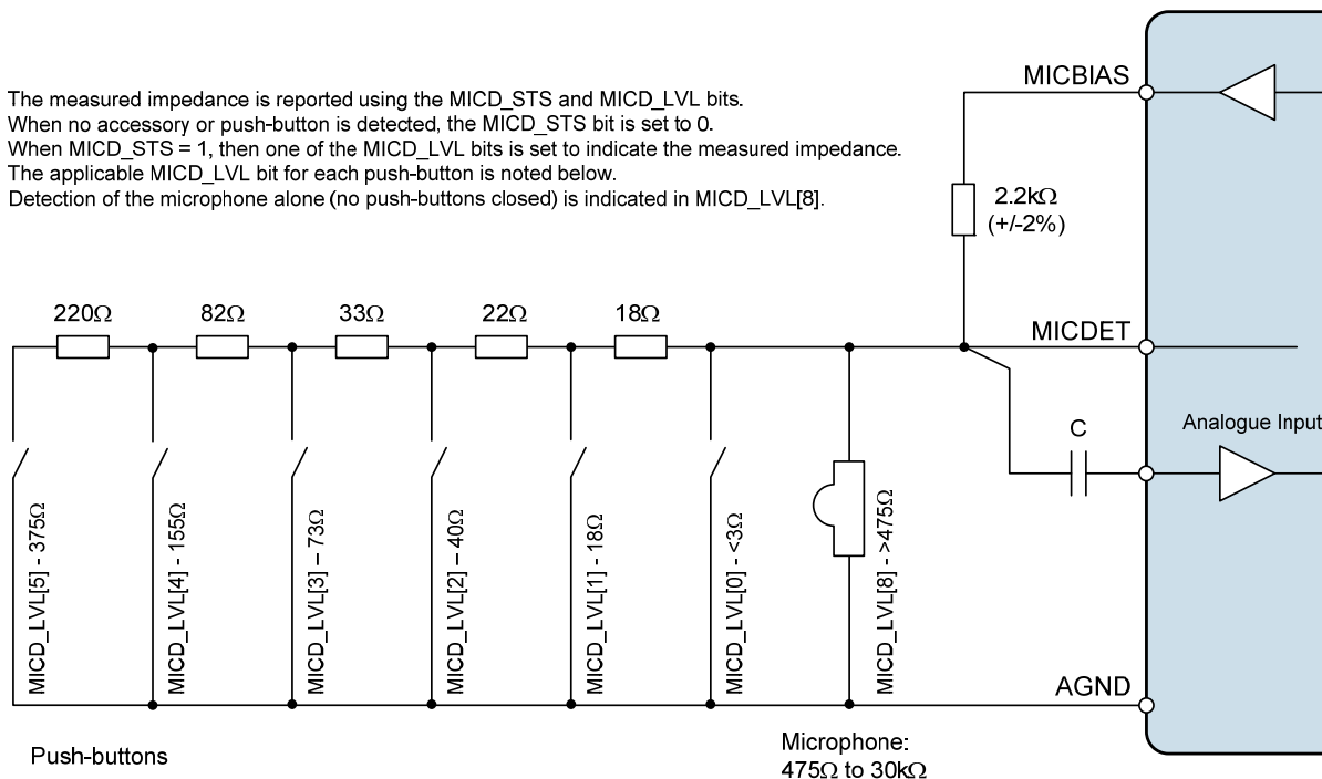
Figure 92 External Accessory Detect Connection
