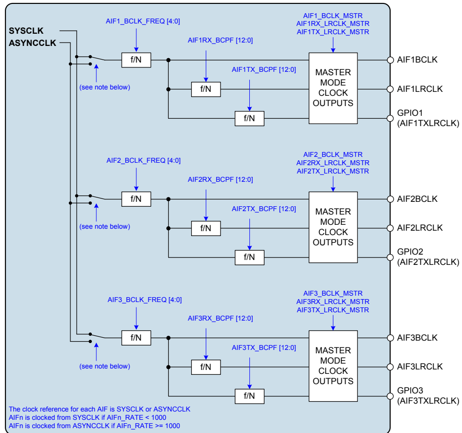
Figure 69 BCLK and LRCLK Control
