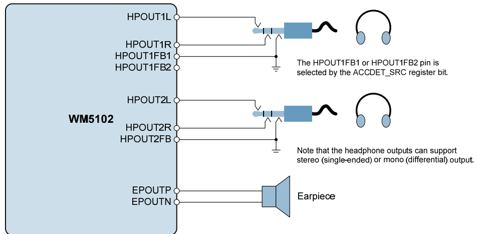
Figure 57 Headphone and Earpiece Connection
