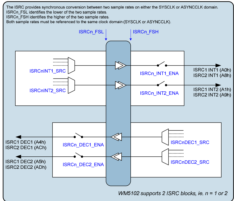
Figure 41 Isochronous Sample Rate Converters (ISRCs)
