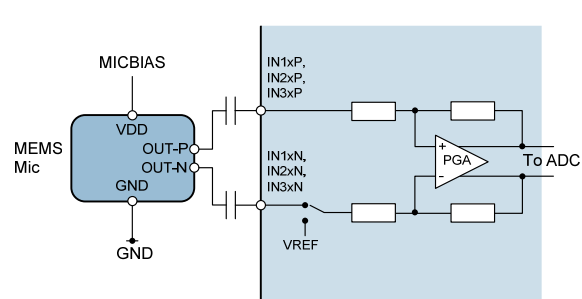
Figure 17 Differential MEMS Input
