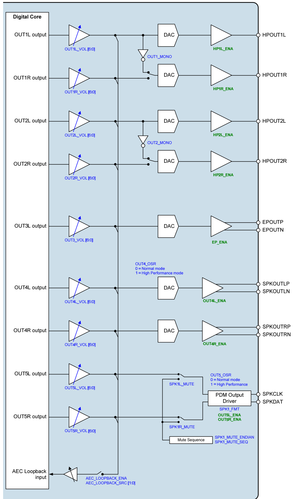
Figure 56 Output Signal Paths
