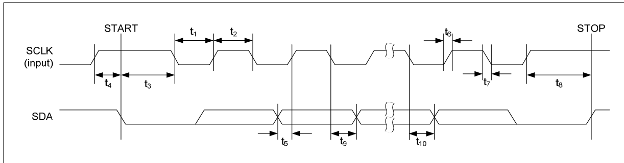
Figure 9 Control Interface Timing - 2-wire (I2C) Control Mode
