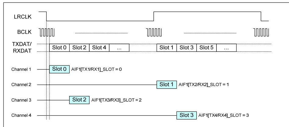
Figure 51 I2S Example
