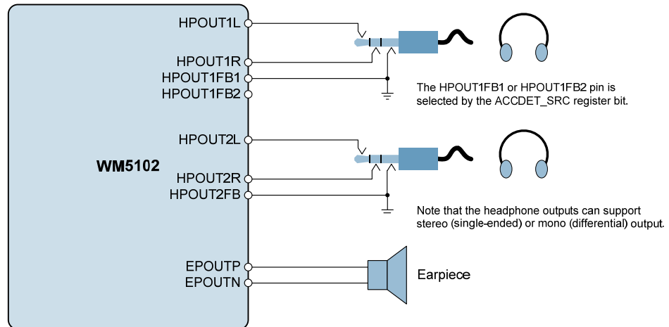
Figure 86 Headphone and Earpiece Connection
