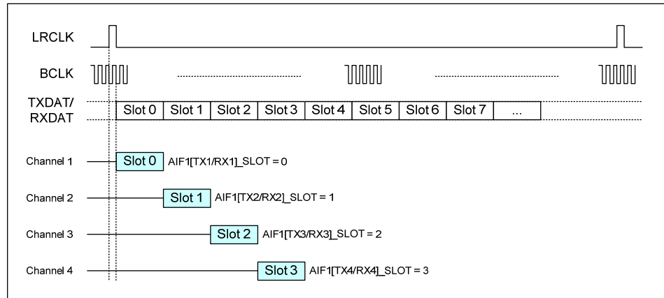
Figure 49 DSP Mode A Example
