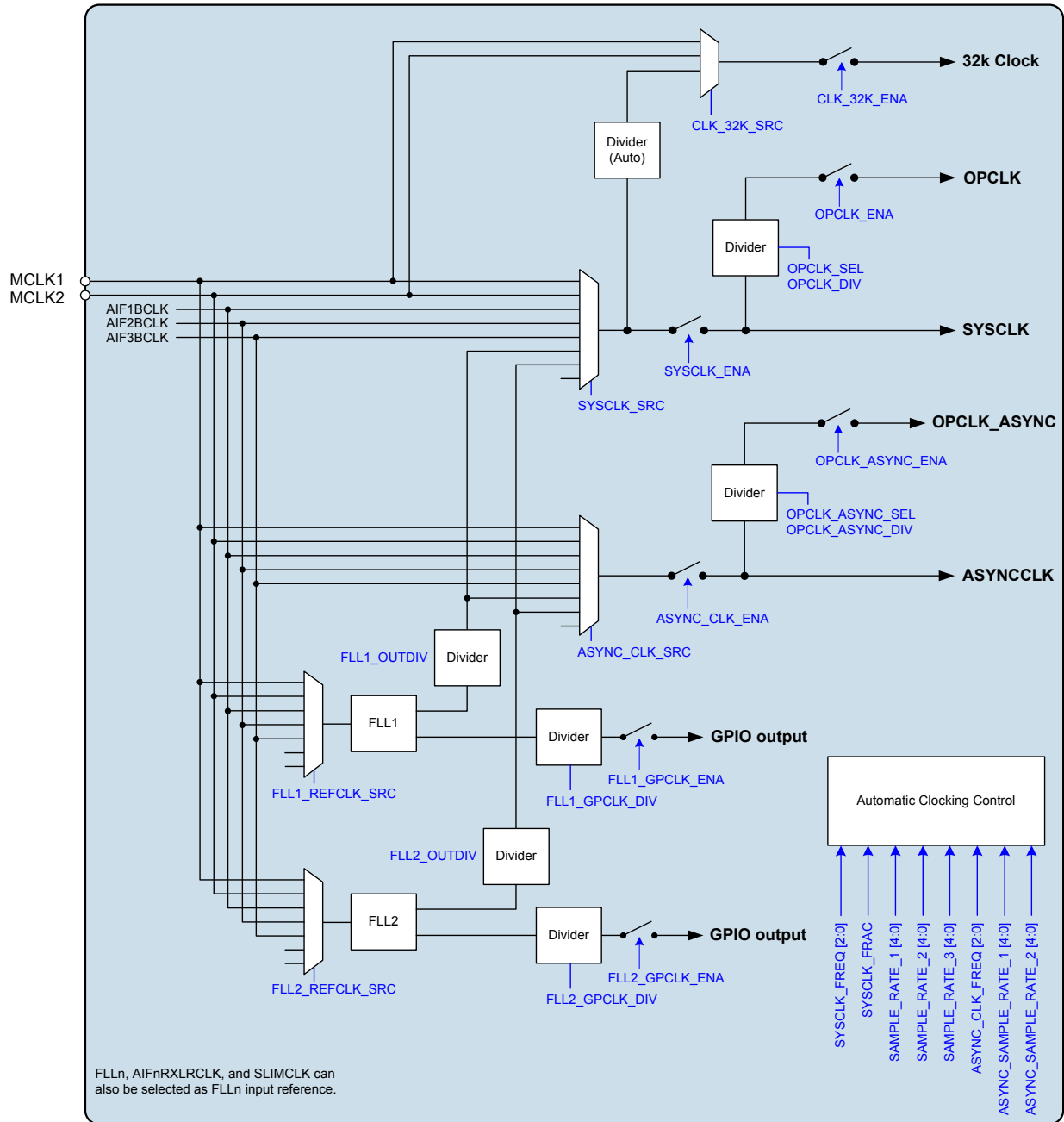
Figure 68 System Clocking
