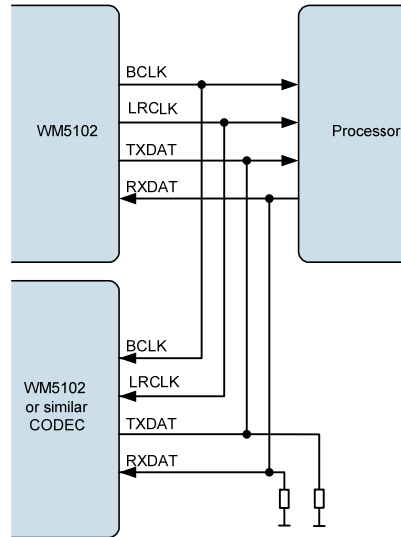
Figure 53 TDM with WM5102 as Master
