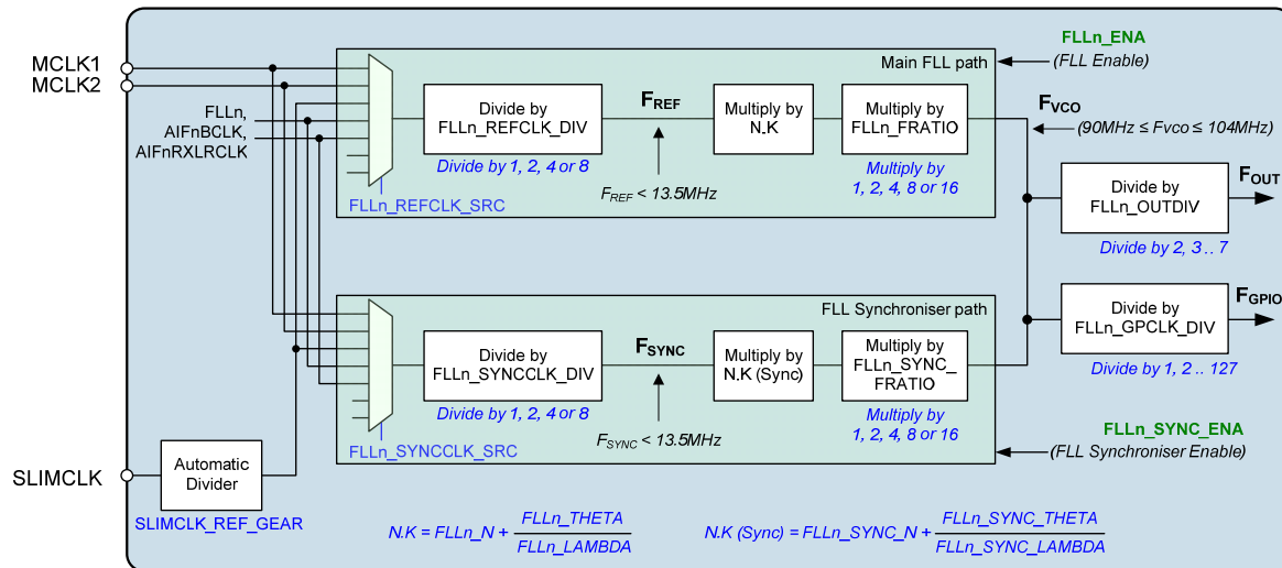
Figure 70 FLL Configuration
