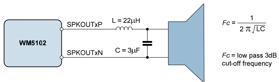
Figure 89 Class D Output Filter Components
