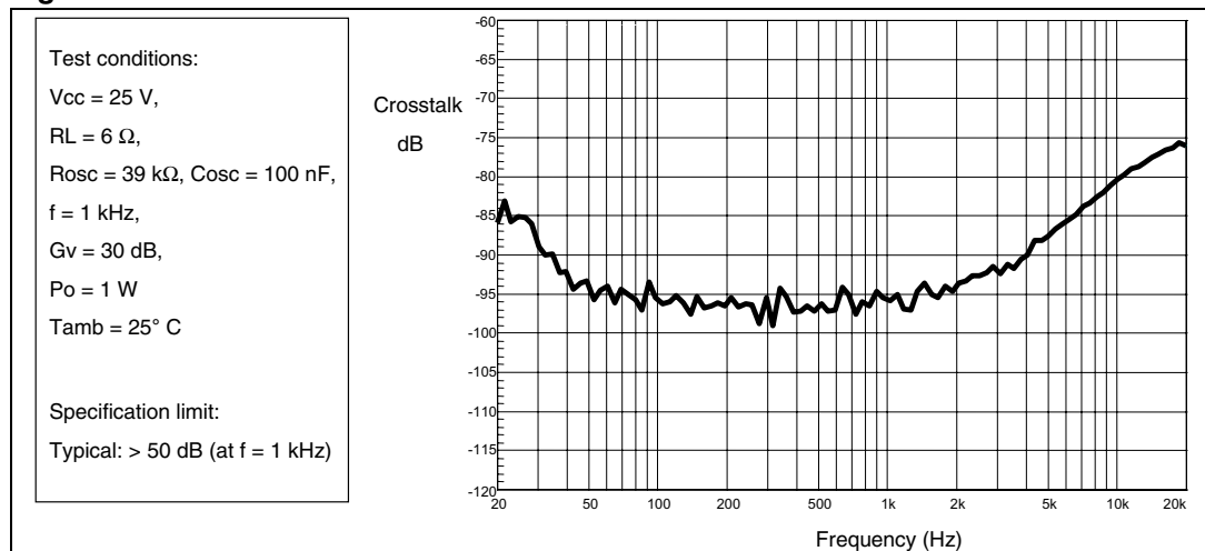
Figure 8. Crosstalk
