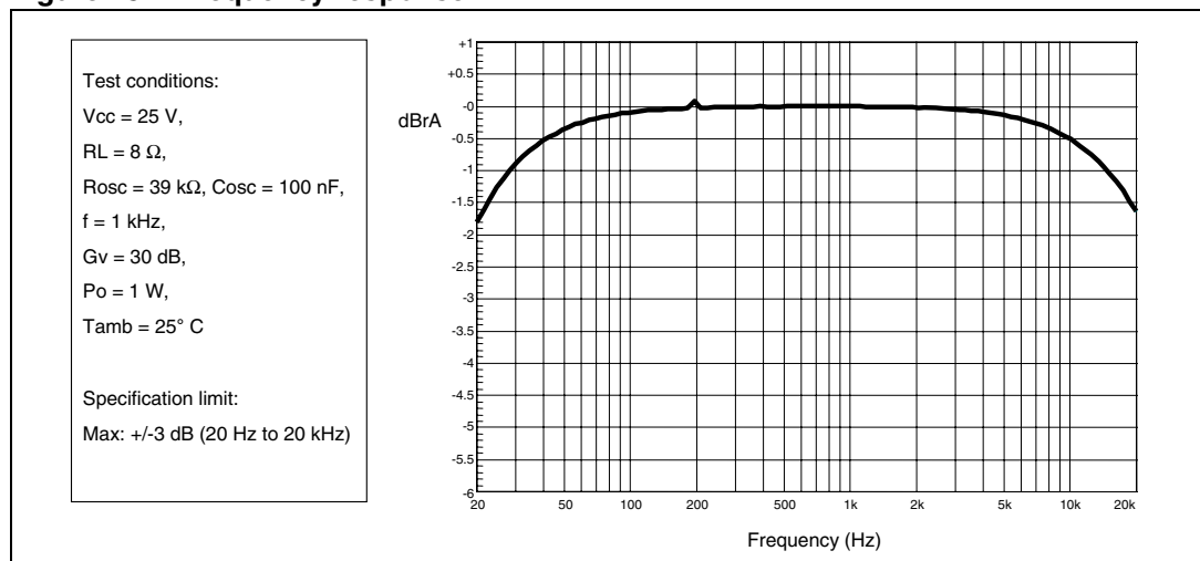
Figure 15. Frequency response
