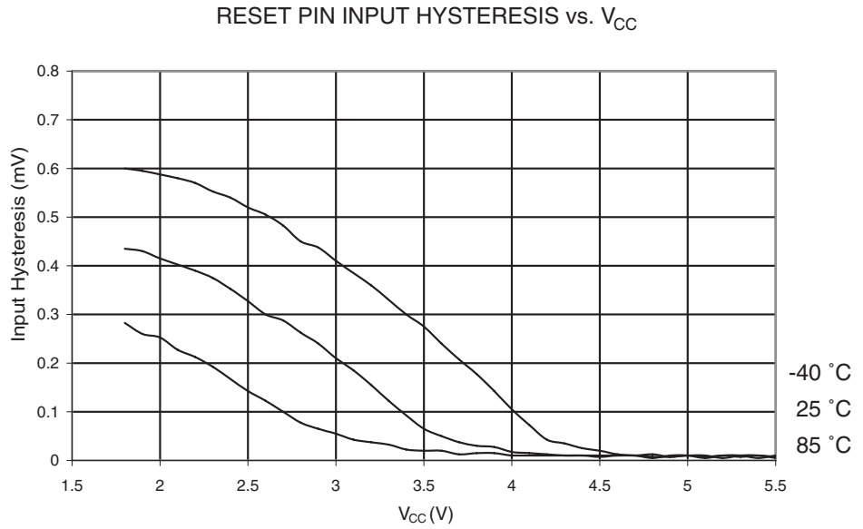
Figure 23-29. Reset Pin Input Hysteresis vs. V_{CC}
