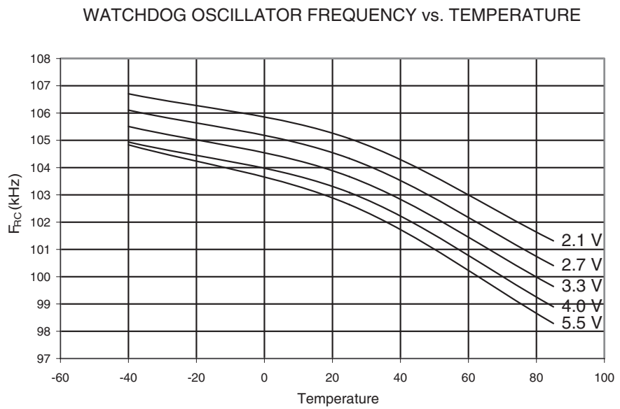
Figure 23-34. Watchdog Oscillator Frequency vs. Temperature
