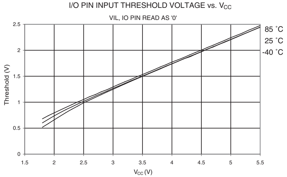
Figure 23-25. I/O Pin Input threshold Voltage vs. V_{CC} ( V_{IL} , IO Pin Read as '0')
