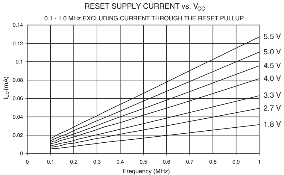
Figure 23-44. Reset Supply Current vs. V_{CC} (0.1 - 1.0 MHz, excluding Current Through the Reset Pull-up)
