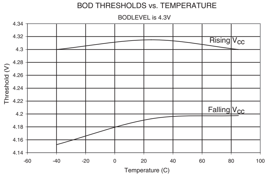
Figure 23-30. BOD Threshold vs. Temperature (BODLEVEL is 4.3V)
