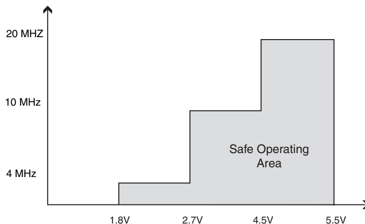
Figure 22-1. Maximum Frequency vs. V_{CC}
