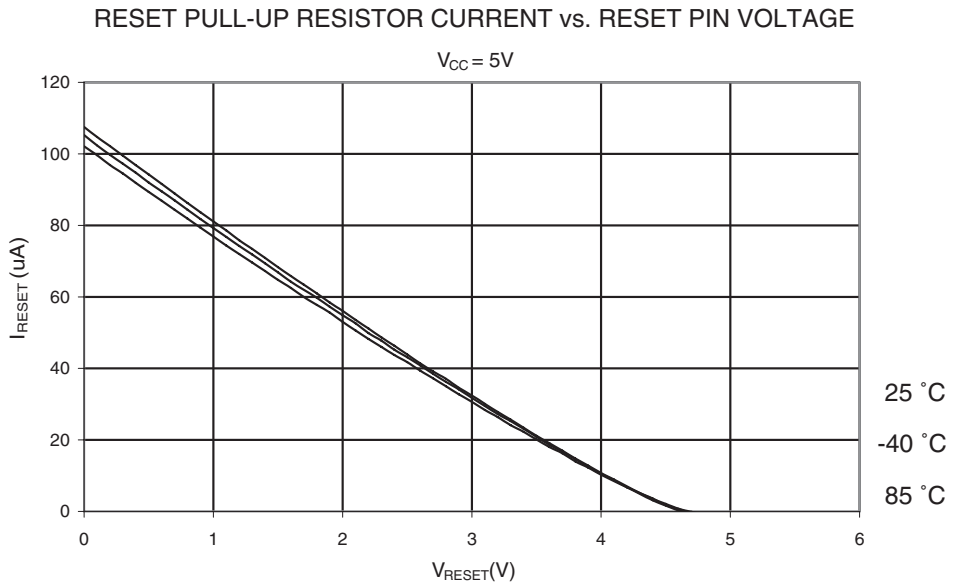
Figure 23-19. Reset Pull-up Resistor Current vs. Reset Pin Voltage ( V_{CC} = 5V )
