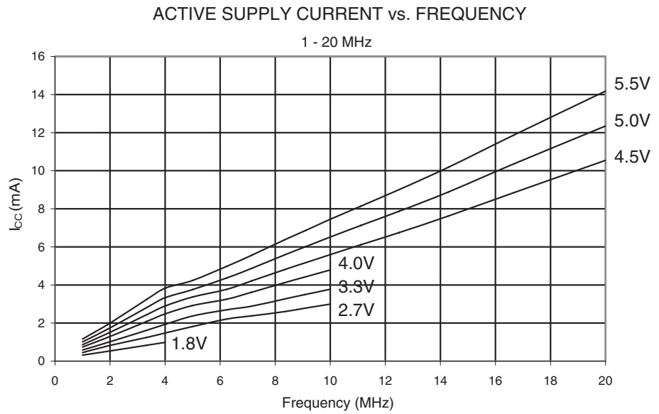
Figure 23-2. Active Supply Current vs. frequency (1 - 20 MHz)
