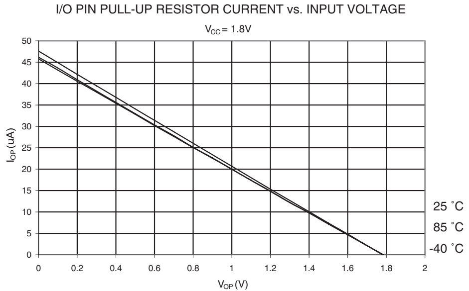
Figure 23-14. I/O pin Pull-up Resistor Current vs. Input Voltage ( V_{CC} = 1.8V )
