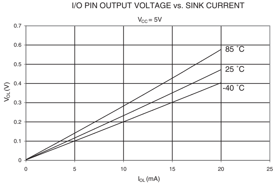
Figure 23-21. I/O pin Output Voltage vs. Sink Current ( V_{CC} = 5V )
