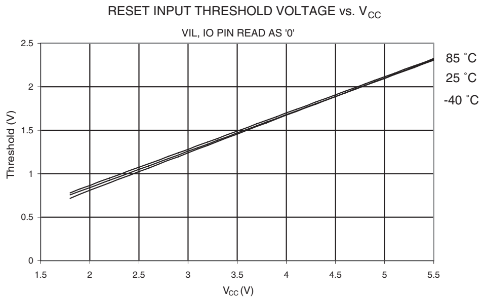
Figure 23-28. Reset Input Threshold Voltage vs. V_{CC} ( V_{IL} , IO pin Read as '0')
