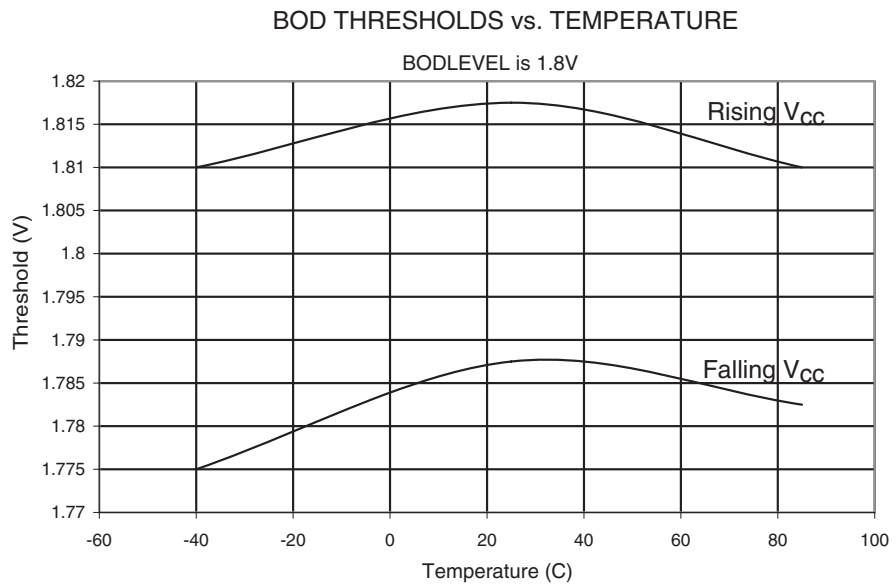
Figure 23-32. BOD Threshold vs. Temperature (BODLEVEL is 1.8V)
