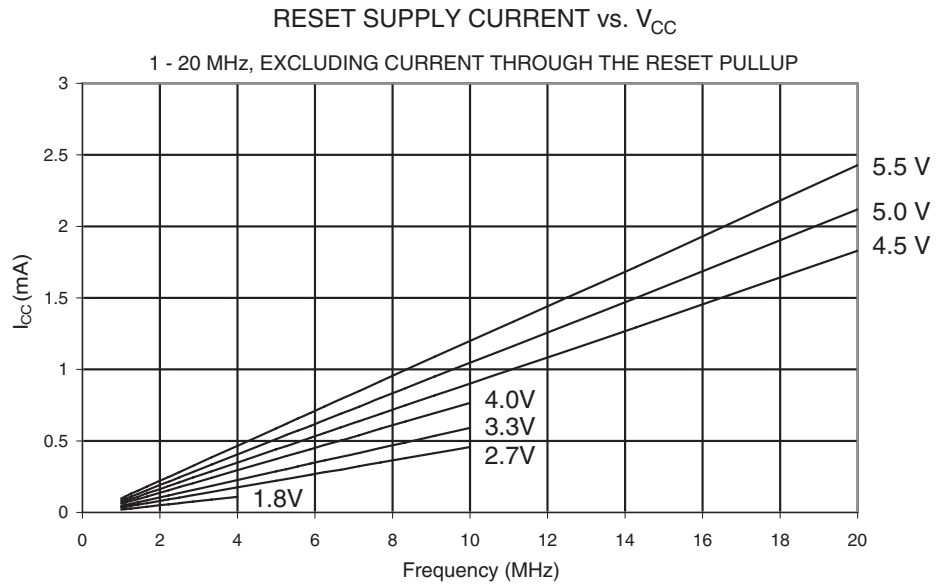
Figure 23-45. Reset Supply Current vs. V_{CC} (1 - 20 MHz, Excluding Current Through the Reset Pull-up)
