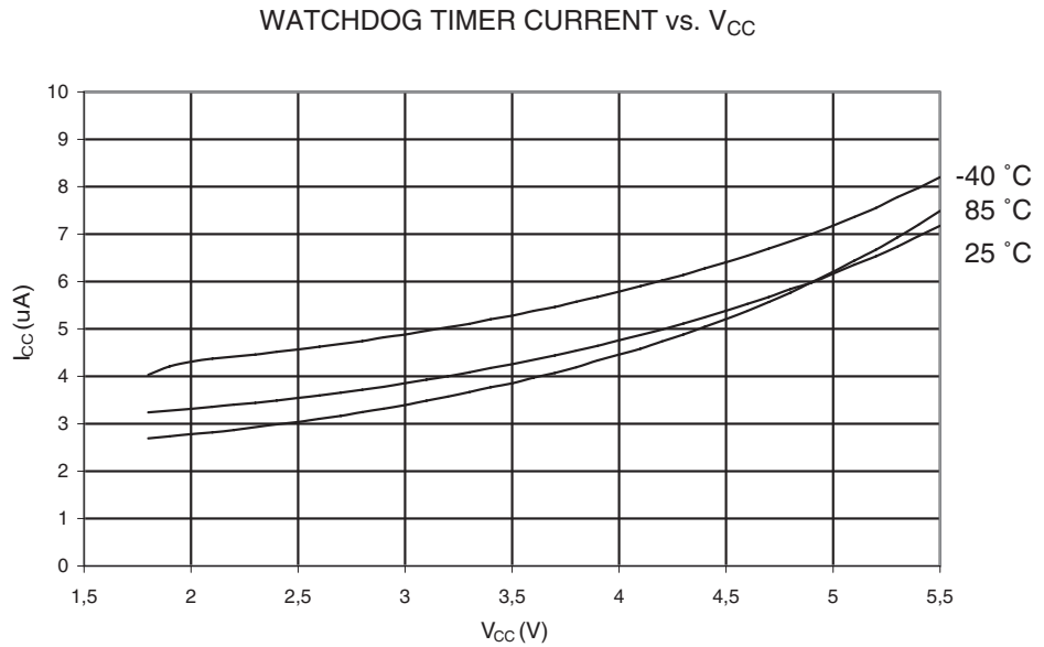
Figure 23-43. Watchdog Timer Current vs. V_{CC}
