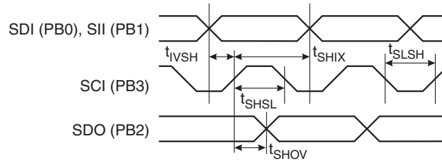
Figure 22-5. High-voltage Serial Programming Timing
