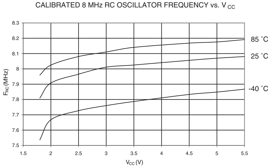
Figure 23-35. Calibrated 8 MHz RC Oscillator Frequency vs. V_{CC}
