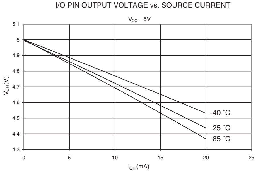
Figure 23-23. I/O Pin output Voltage vs. Source Current ( V_{CC} = 5V )
