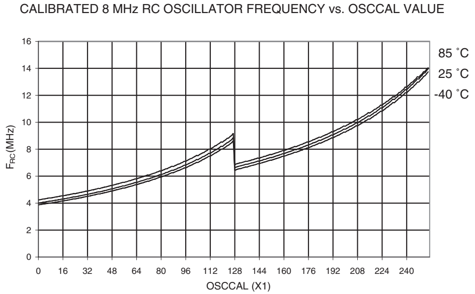
Figure 23-37. Calibrated 8 MHz RC Oscillator Frequency vs. OSCCAL Value
