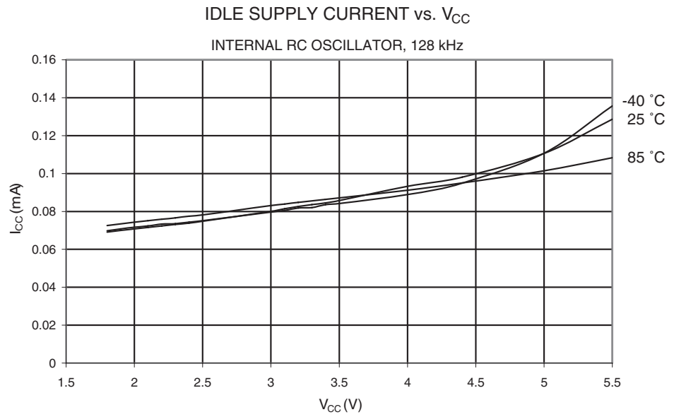
Figure 23-10. Idle Supply Current vs. V_{CC} (Internal RC Oscillator, 128 MHz)
