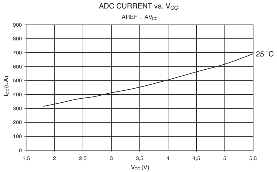
Figure 23-38. ADC Current vs. V CC
