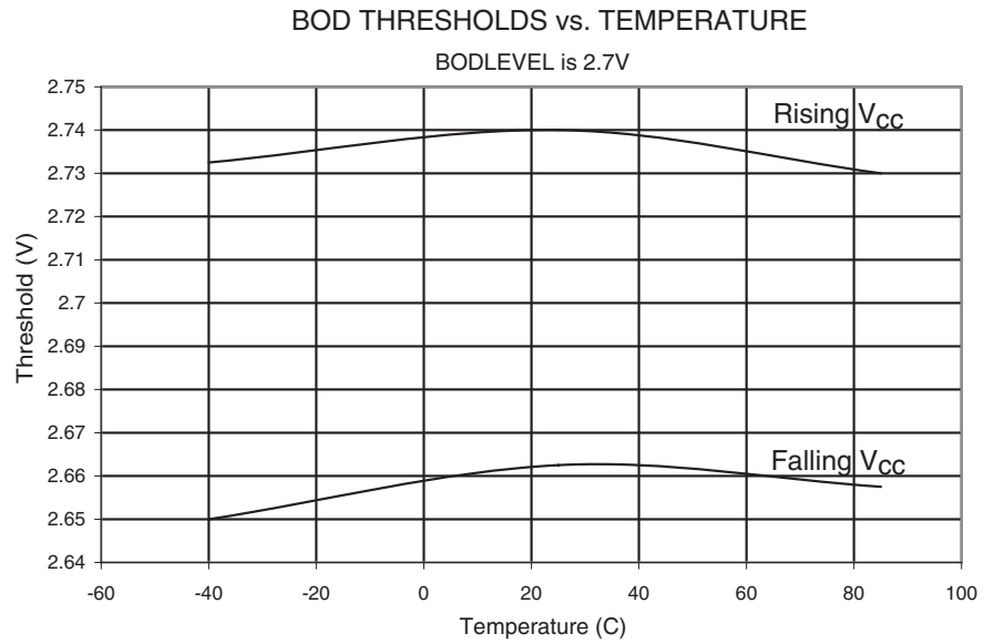
Figure 23-31. BOD Threshold vs. Temperature (BODLEVEL is 2.7V)
