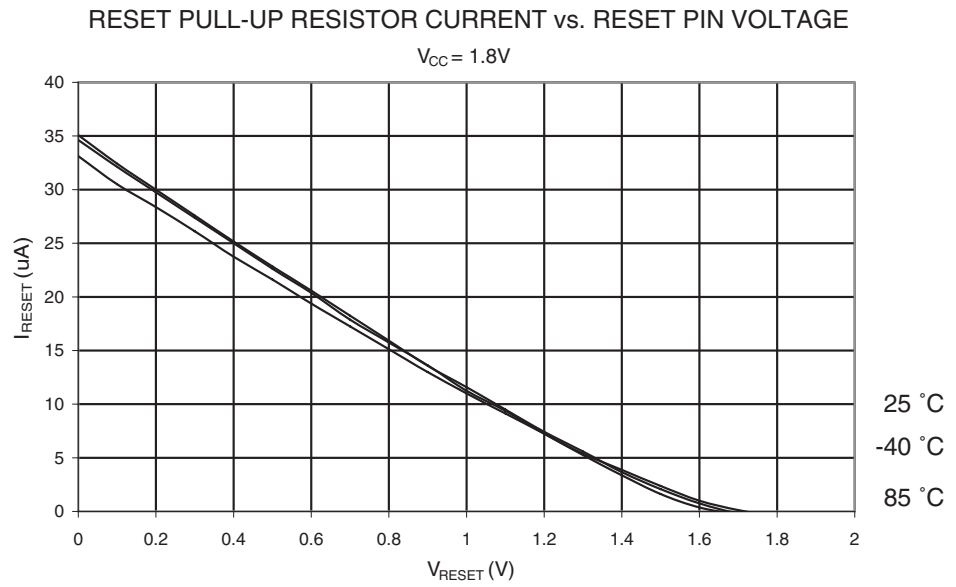
Figure 23-17. Reset Pull-up Resistor Current vs. Reset Pin Voltage ( V_{CC} = 1.8V )
