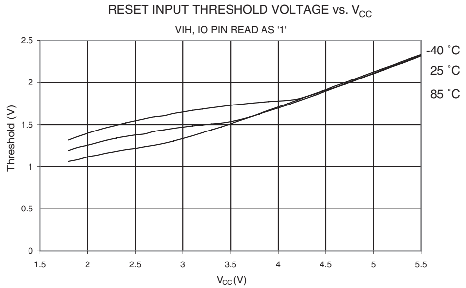
Figure 23-27. Reset Input Threshold Voltage vs. V_{CC} ( V_{IH} , IO Pin Threshold as '1')
