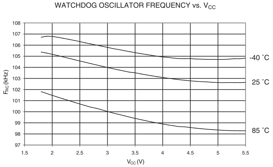
Figure 23-33. Watchdog Oscillator Frequency vs. V_{CC}
