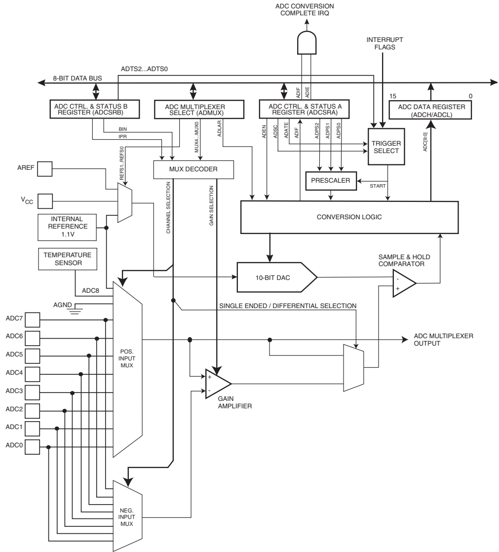
Figure 18-1. Analog to Digital Converter Block Schematic
