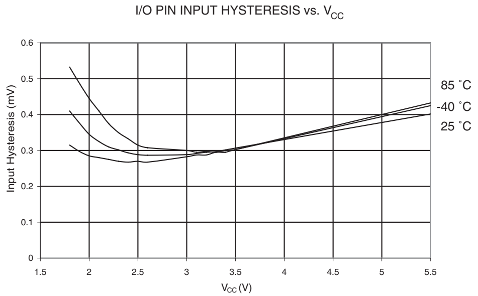
Figure 23-26. I/O Pin Input Hysteresis vs. V_{CC}
