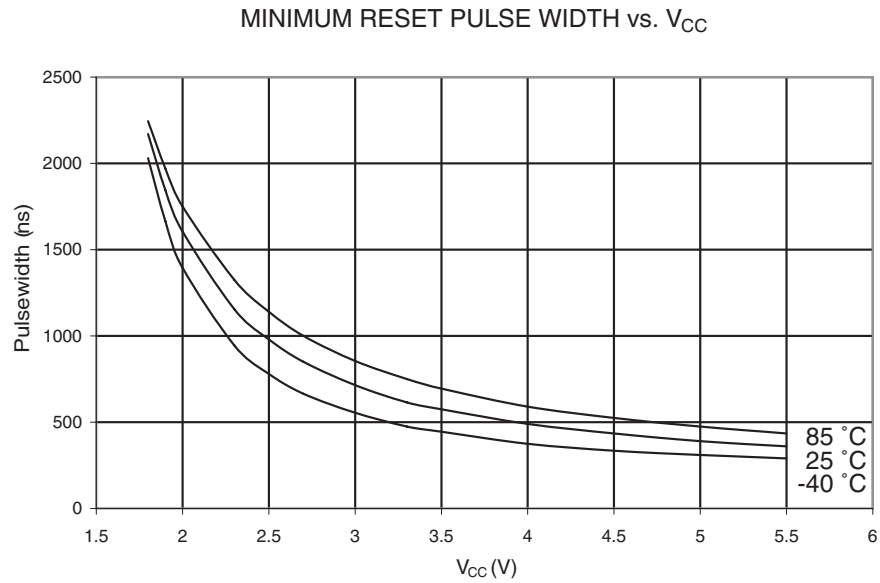
Figure 23-46. Minimum Reset Pulse Width vs. V_{CC}
