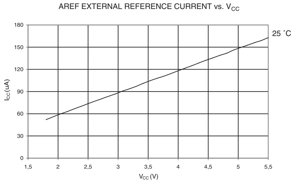
Figure 23-39. AREF External Reference Current vs. V_{CC}
