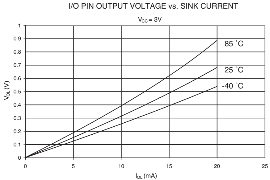
Figure 23-20. I/O Pin Output Voltage vs. Sink Current ( V_{CC} = 3V )
