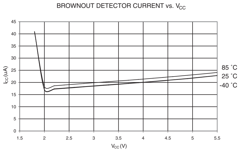
Figure 23-42. Brownout Detector Current vs. V_{CC}
