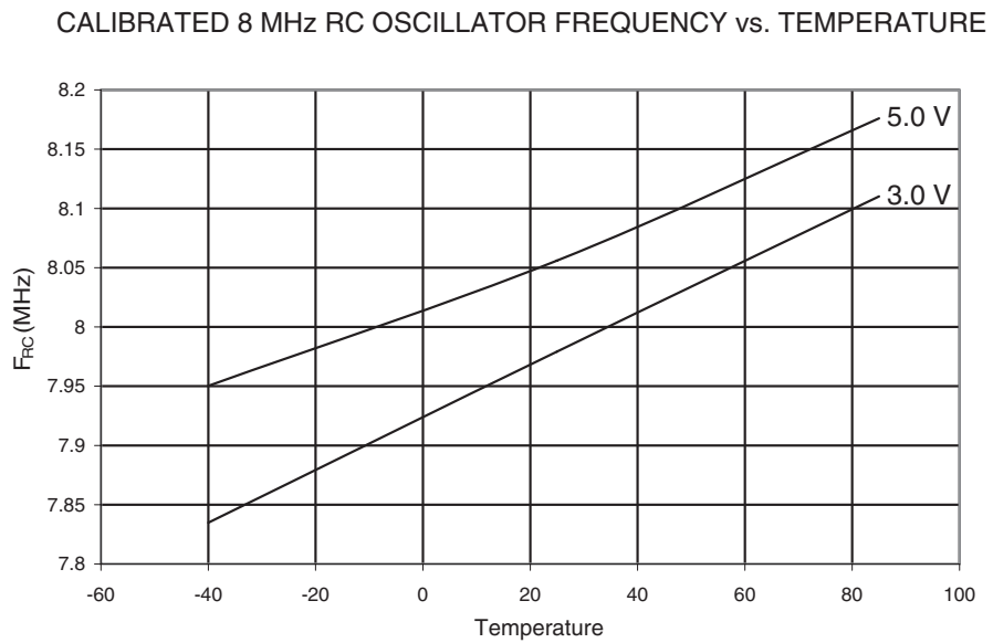
Figure 23-36. Calibrated 8 MHz RC oscillator Frequency vs. Temperature
