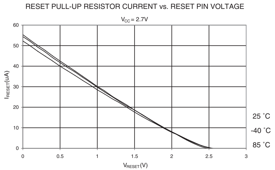
Figure 23-18. Reset Pull-up Resistor Current vs. Reset Pin Voltage ( V_{CC} = 2.7V )
