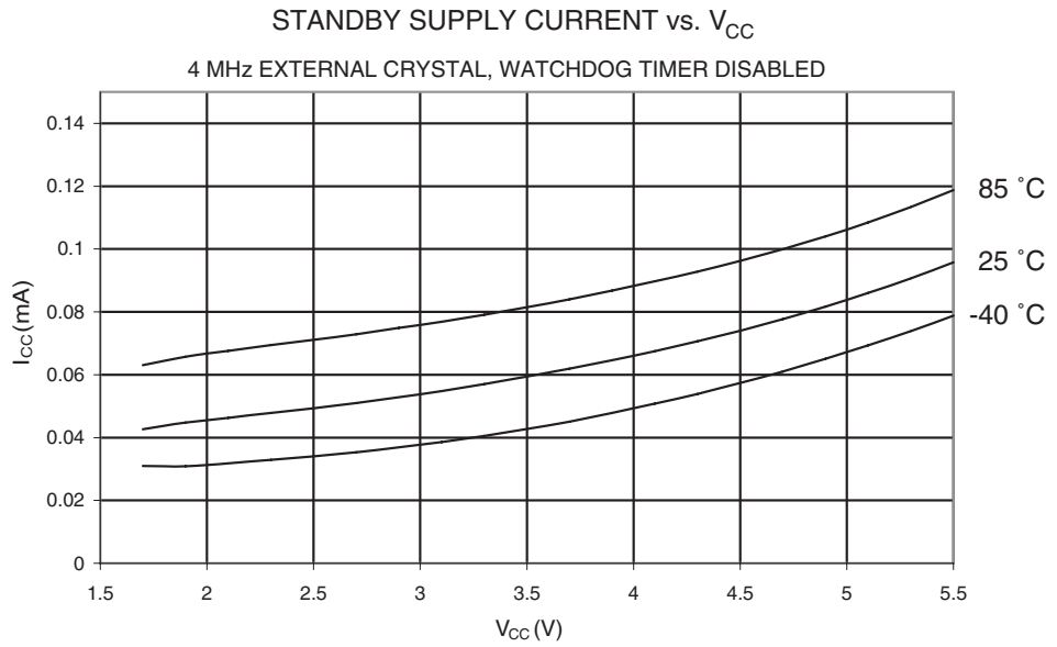
Figure 23-13. Standby Supply Current vs. V_{CC} (4 MHz External Crystal, Watchdog Timer Disabled)
