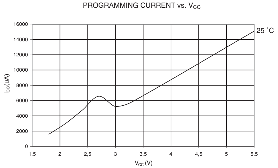
Figure 23-41. Programming Current vs. V_{CC}
