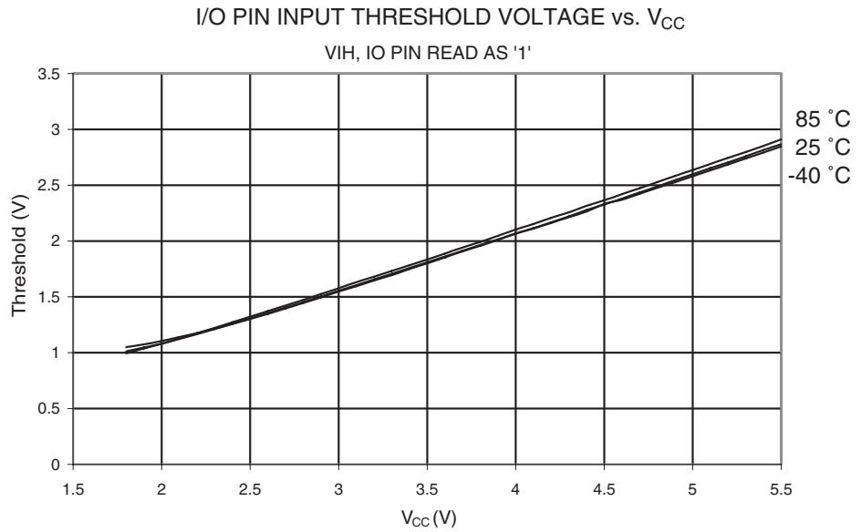
Figure 23-24. I/O Pin Input Threshold Voltage vs. V_{CC} ( V_{IH} , IO Pin Read as '1')
