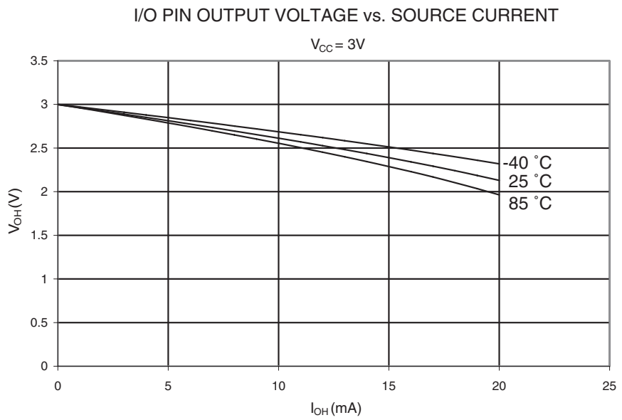
Figure 23-22. I/O Pin Output Voltage vs. Source Current ( V_{CC} = 3V )
