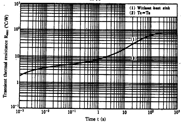
R_{th}(t) - t
