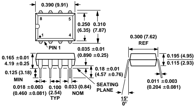
Mini-DIP (N-8)
