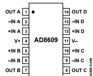
Figure 5. 14-Lead SOIC (R Suffix)
