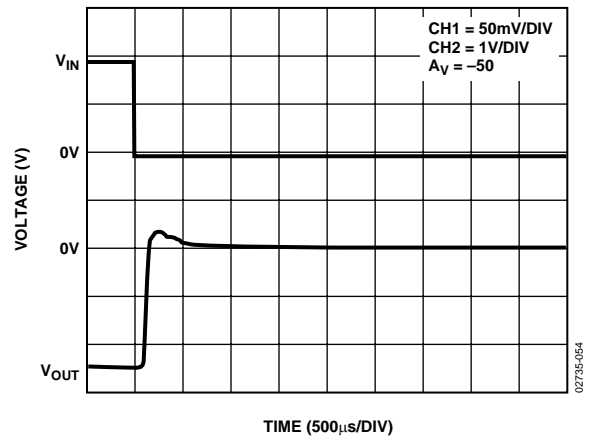
Figure 57. Positive Input Overload Recovery for LTC2050
