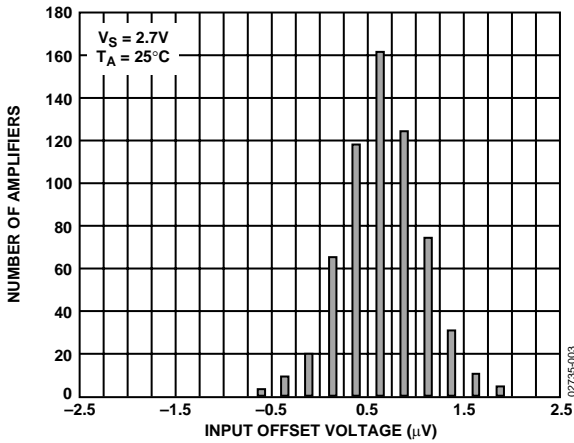
Figure 5. Input Offset Voltage Distribution at 2.7 V
