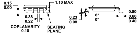
Figure 62. 8-Lead Mini Small Outline Package [MSOP] (RM-8) Dimensions shown in millimeters
