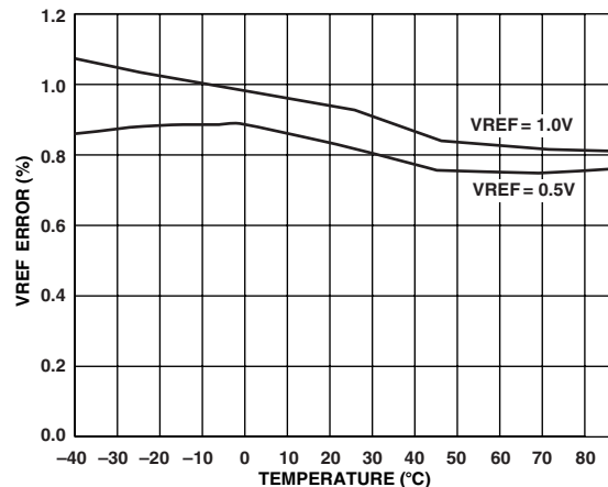
Figure 14. Typical VREF Drift
