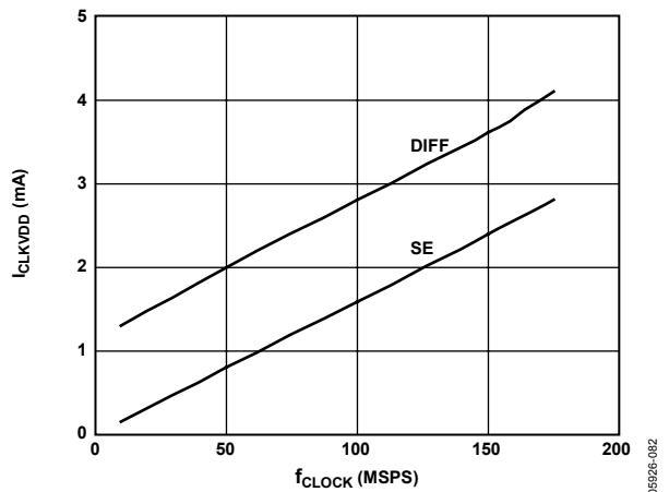
Figure 86. I_{CLKVDD} vs. f_{CLOCK} @ CLKVDD = 3.3 V
