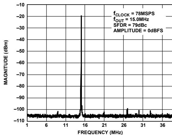
Figure 24. Single-Tone SFDR
