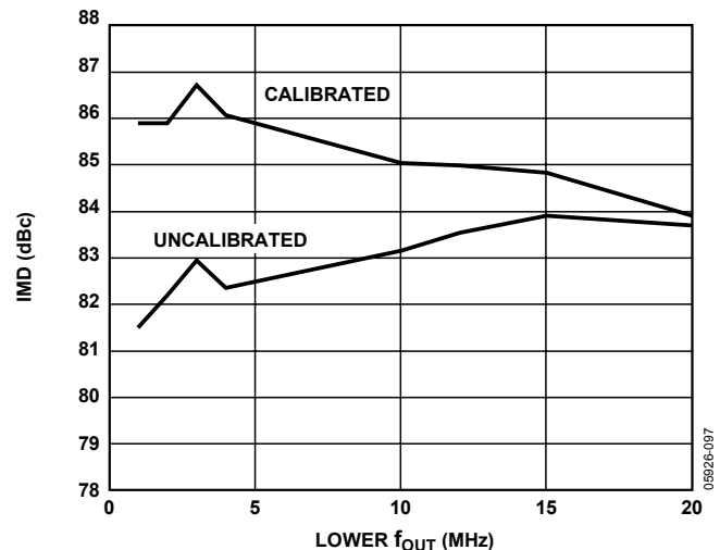
Figure 89. IMD vs. f_{OUT} @ 175 MSPS and I_{OUTFS} = 2 mA
