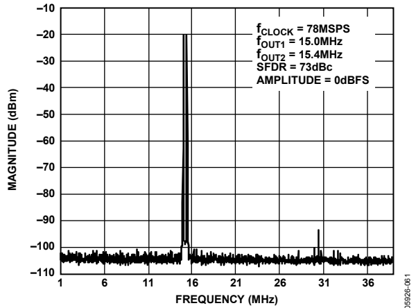
Figure 55. AD9705 Dual-Tone SFDR
