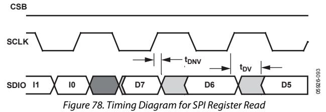
Figure 78. Timing Diagram for SPI Register Read
