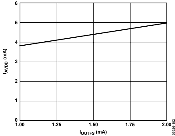
Figure 83. I_{AVDD} vs. I_{OUTFS} @ AVDD = 1.8 V
