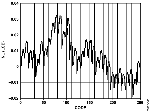
Figure 59. AD9704 Typical Uncalibrated INL
