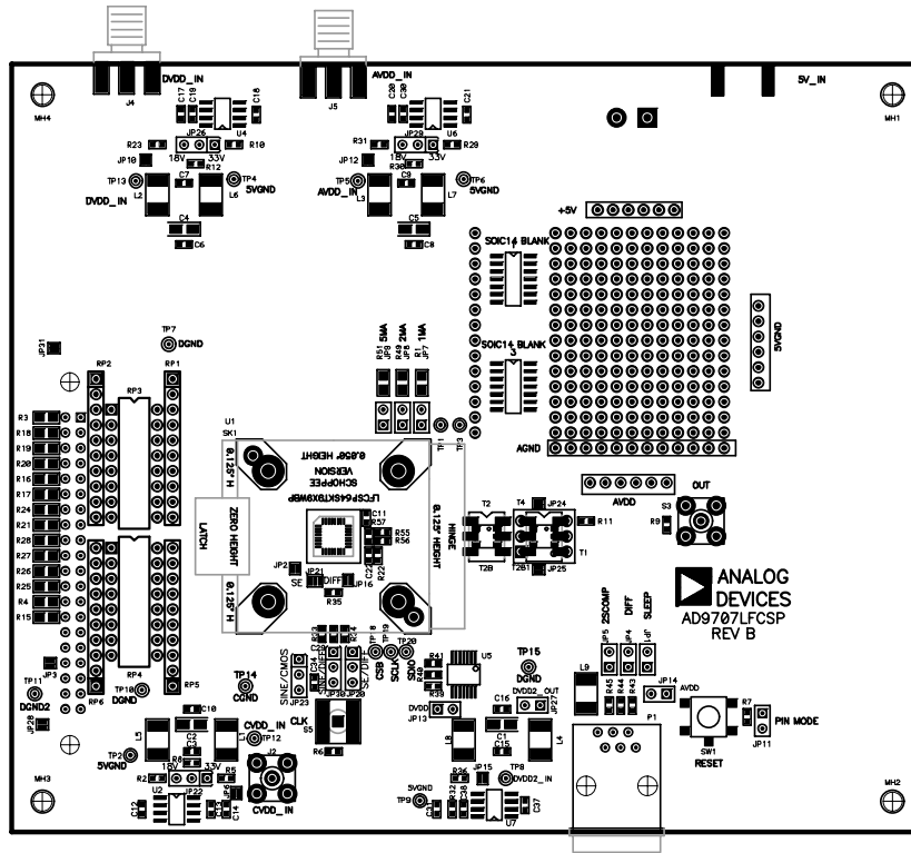
Figure 98. Assembly—Primary Side
