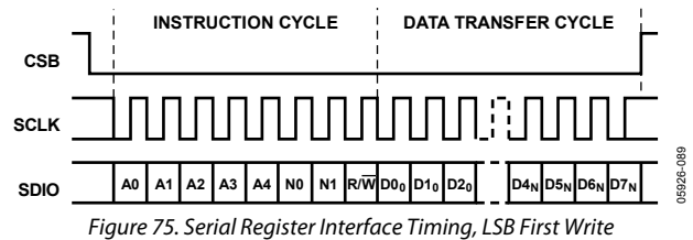
Figure 75. Serial Register Interface Timing, LSB First Write
