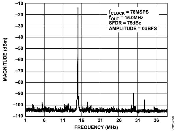
Figure 54. AD9705 Single-Tone SFDR
