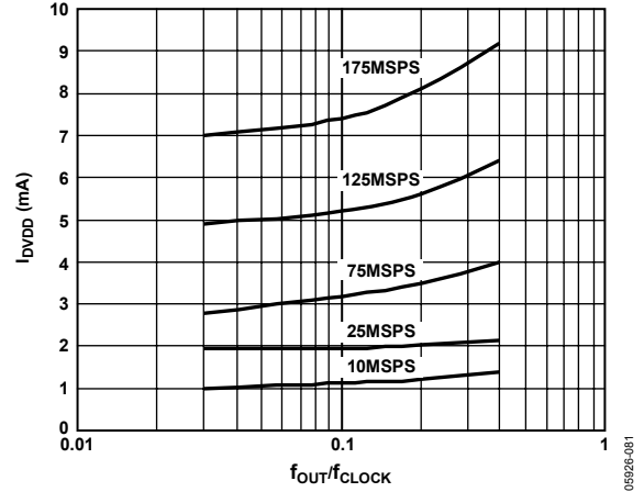
Figure 84. I_{DVDD} vs. f_{OUT}/f_{CLOCK} Ratio @ DVDD = 3.3 V
