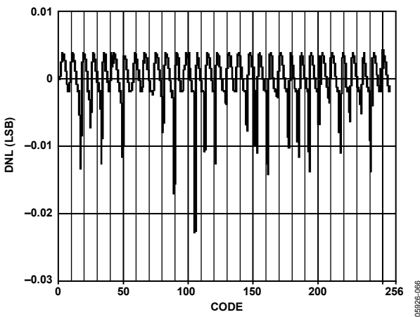
Figure 60. AD9704 Typical Uncalibrated DNL
