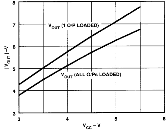
Figure 7. Transmitter Output Voltage vs. V_{CC}
