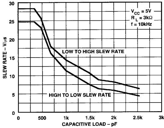
Figure 5. Transmitter Slew Rate vs. Load Capacitance
