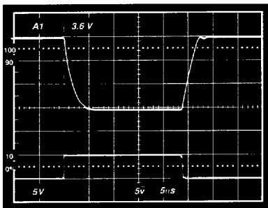
Figure 6. Transmitter Fully Loaded Slew Rate
