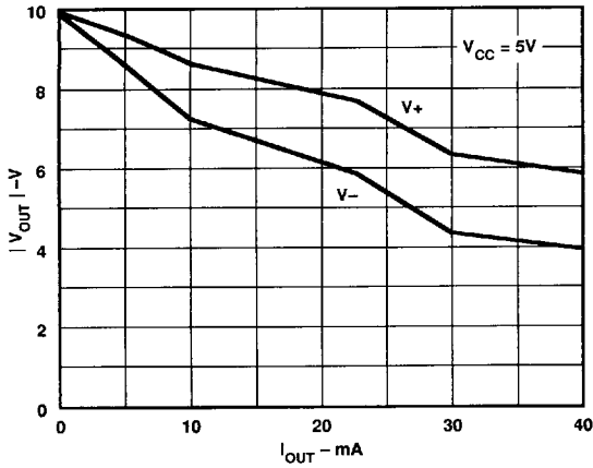
Figure 4. Charge Pump V_+ , V_- vs. Current
