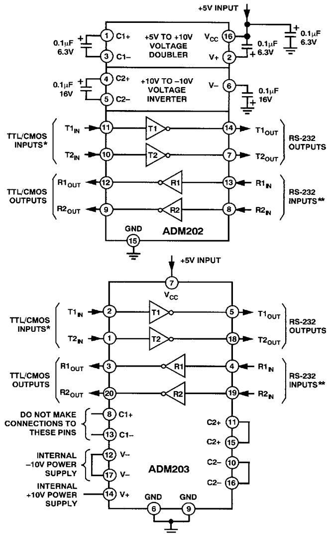
Figure 1. Typical Operating Circuits
