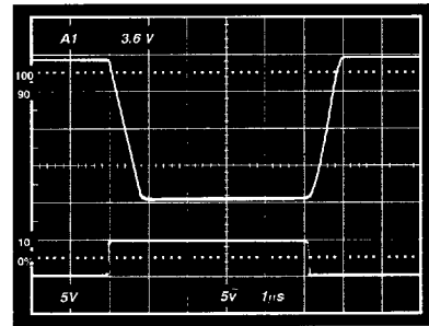
Figure 9. Transmitter Unloaded Slew Rate
