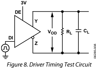
Figure 8. Driver Timing Test Circuit
