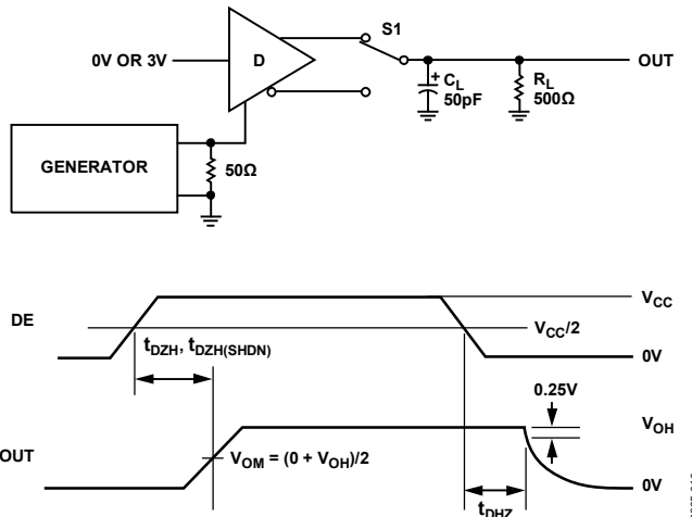
Figure 10. Driver Enable and Disable Times ( t_{DZH} , t_{DZH} , t_{DZH(SHDN)} )
