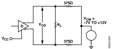
Figure 8. Differential Output Voltage Drivers with Varying Common-Mode Voltage
